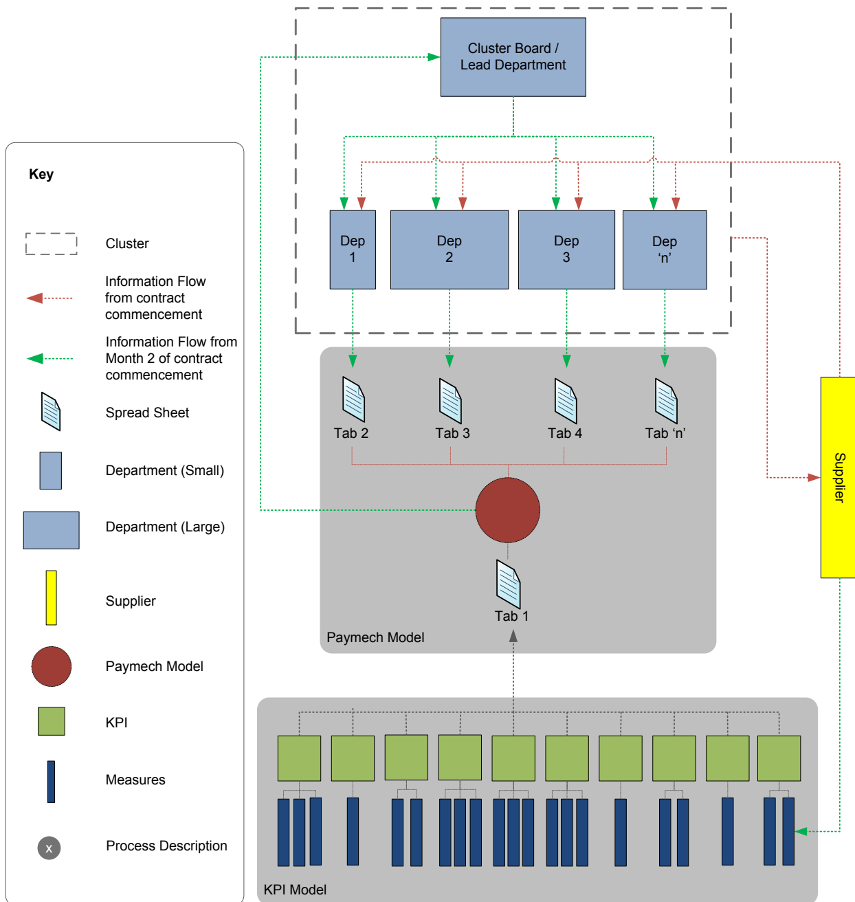
Figure 4.1 Purchase-to-Pay Process
