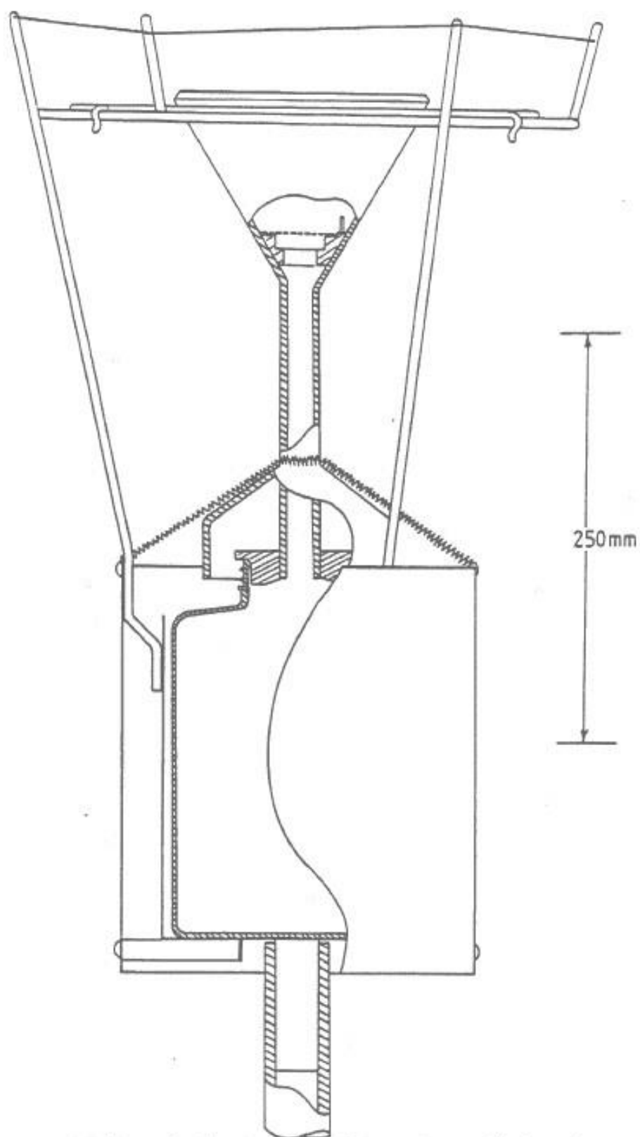
Fig.2 Precipitation Collector for Secondary Network. Details of Sampling Head.
