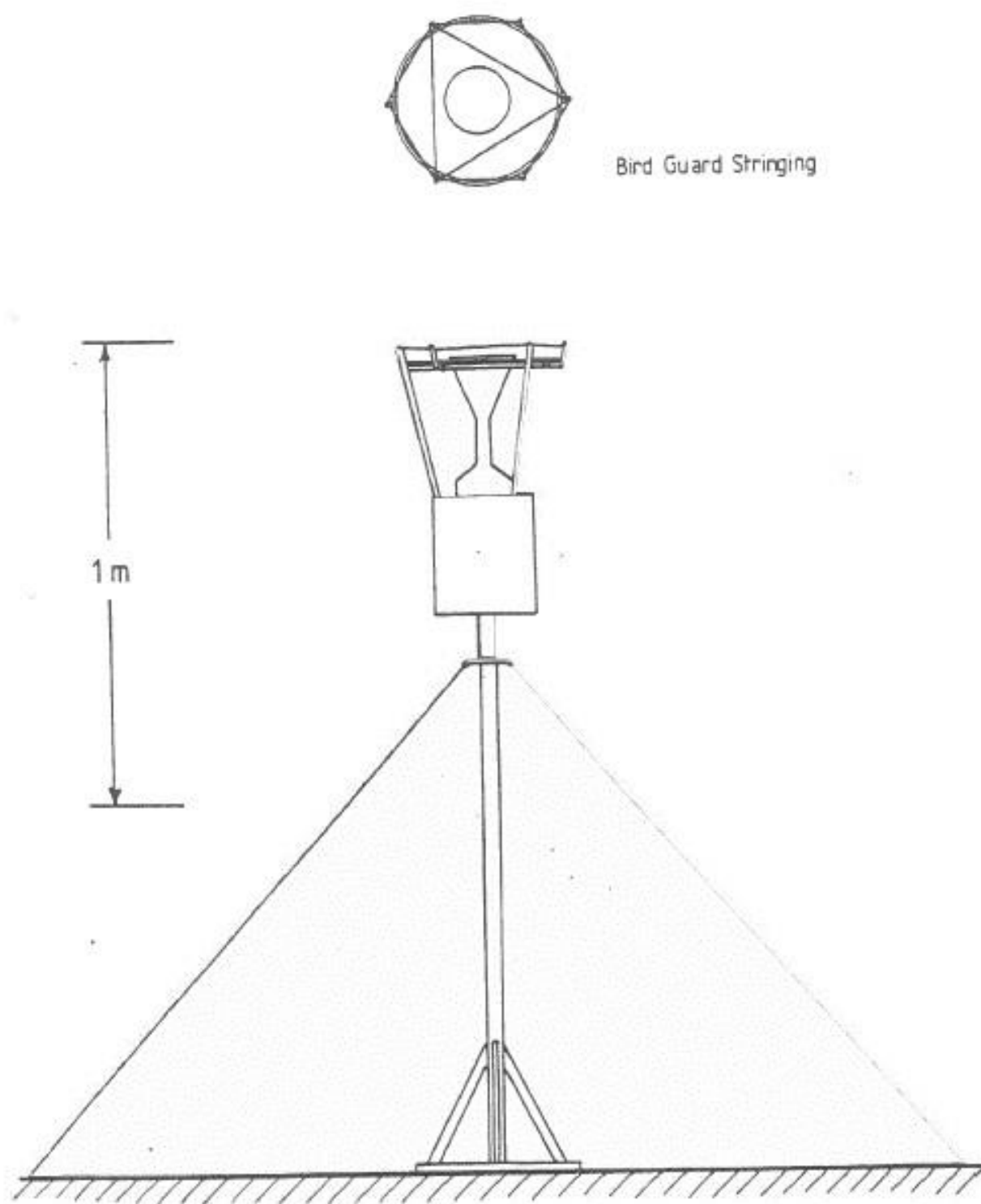
Fig.1 Precipitation Collector for Secondary Network
