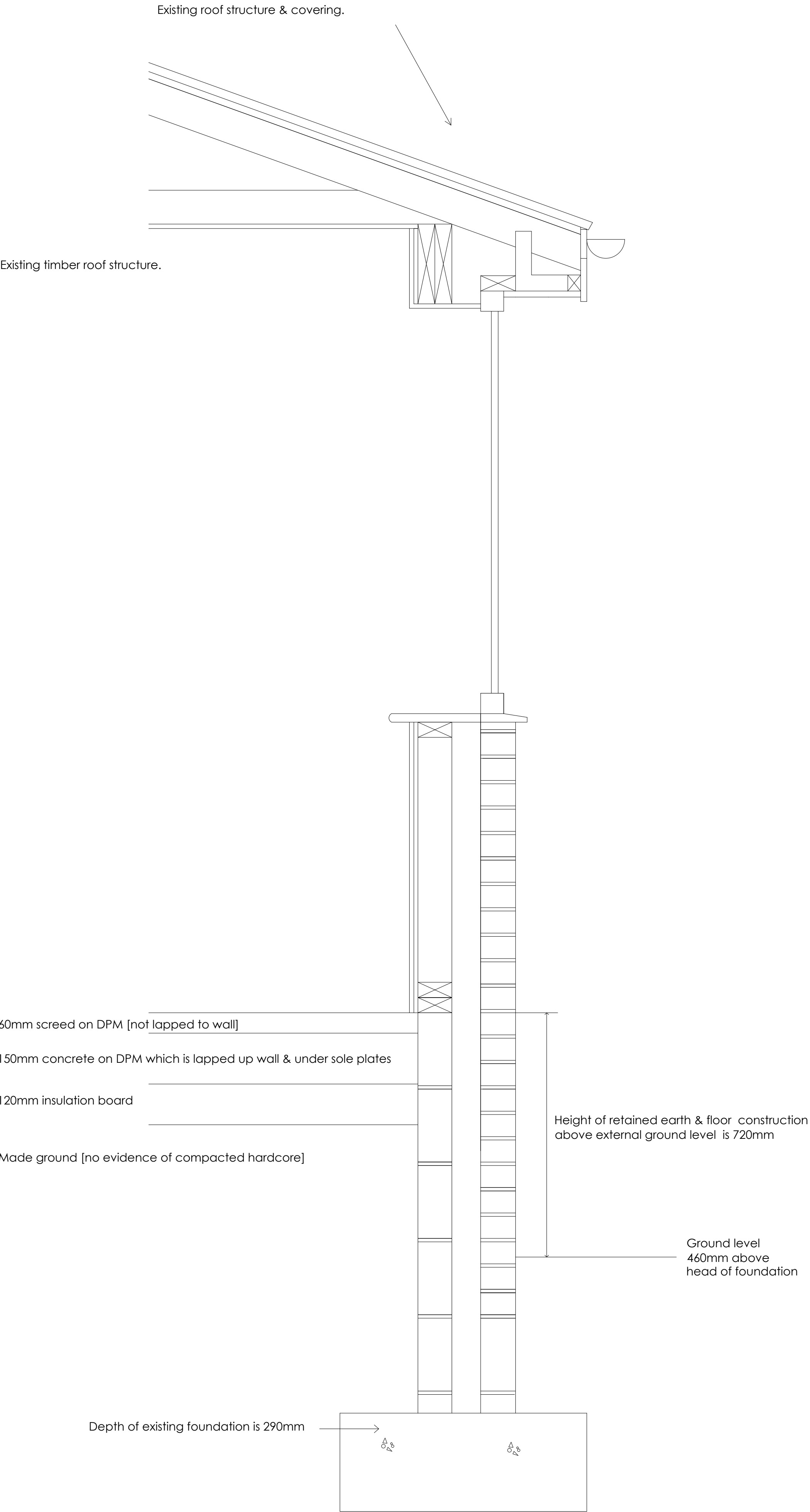
EXISTING SECTION B-B [CONFERENCE ROOM]
