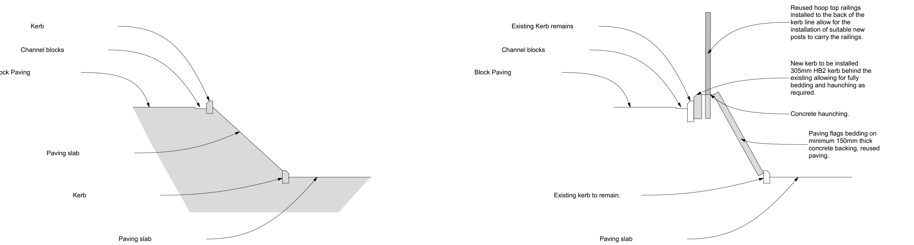
Existing section
