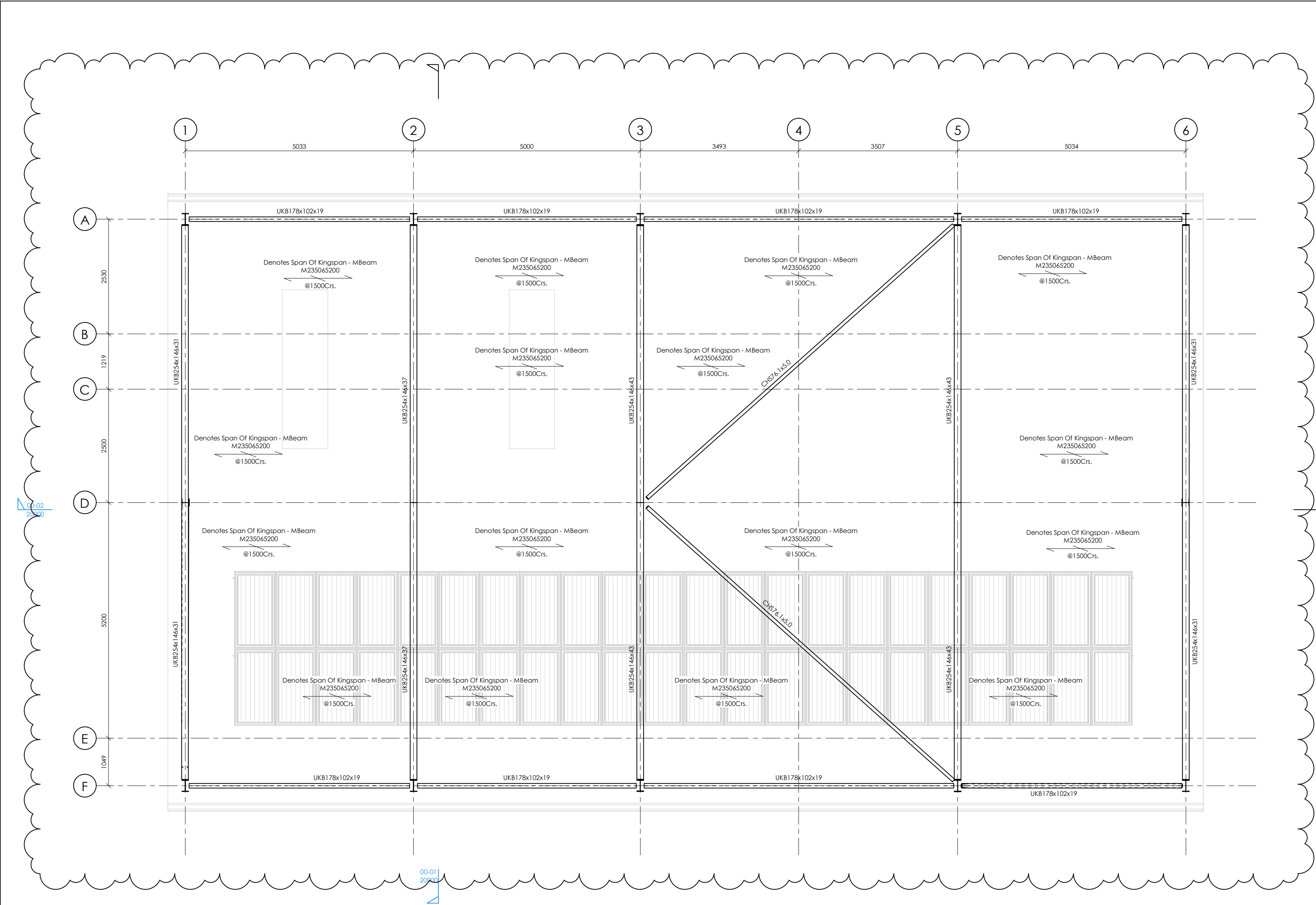
ROOF STRUCTURE LAYOUT 1 : 50
