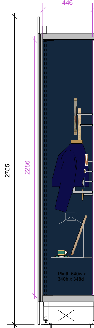
SIDE ELEVATION
