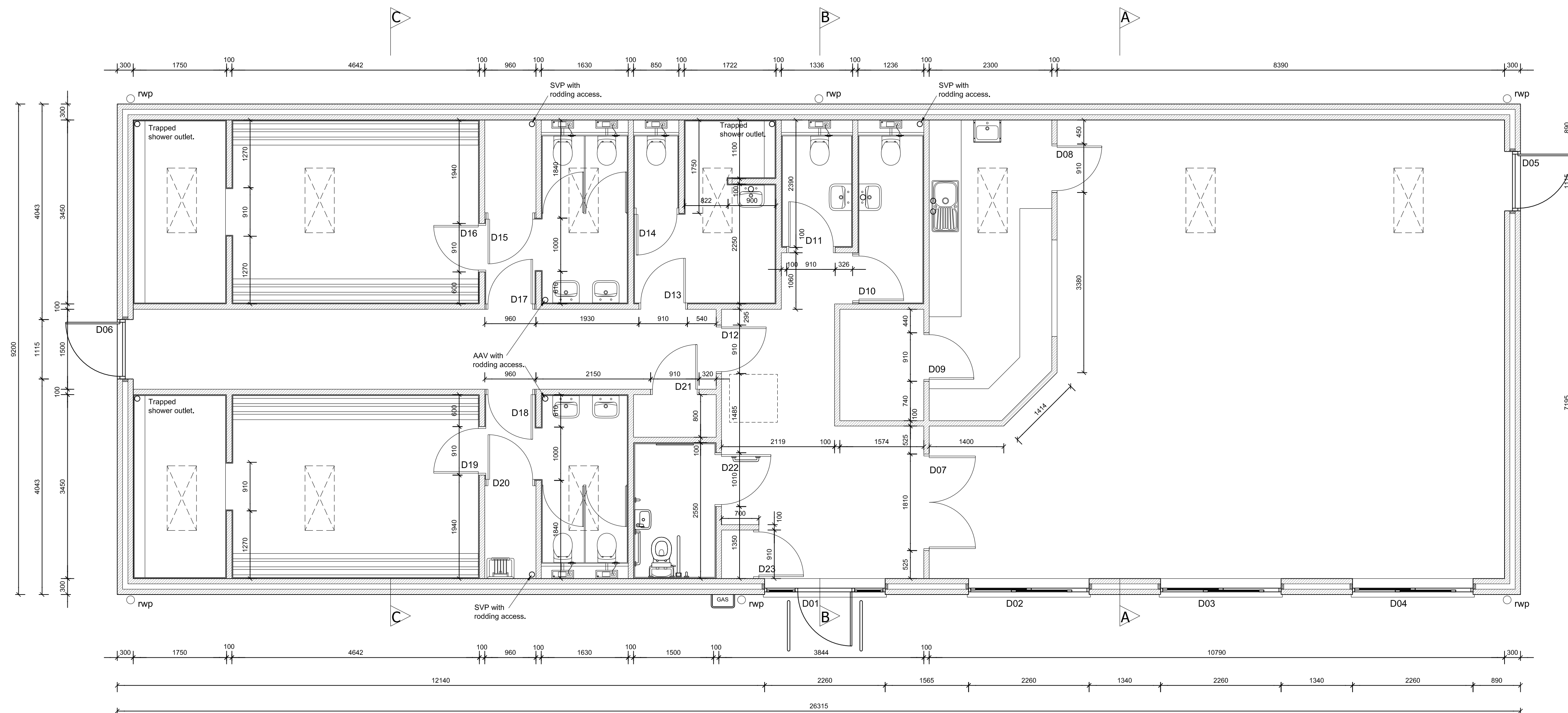
SETTING OUT PLAN
