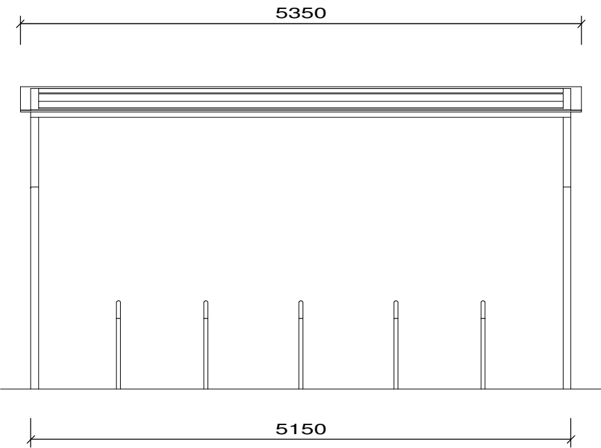
FRONT ELEVATION OF CYCLE STORE 1:50
