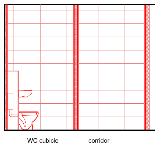
WC cubicles north & south facing elevation as proposed 1:50
