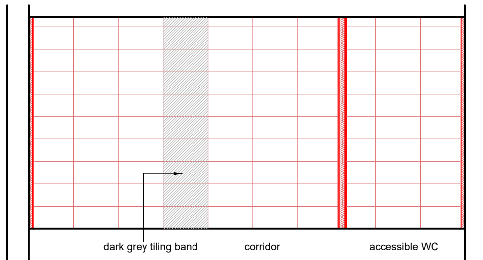
WC corridor wall west facing elevation as proposed 1:50
