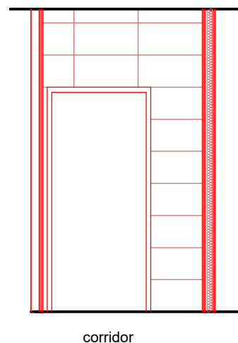
WC corridor wall north facing elevation as proposed 1:50
