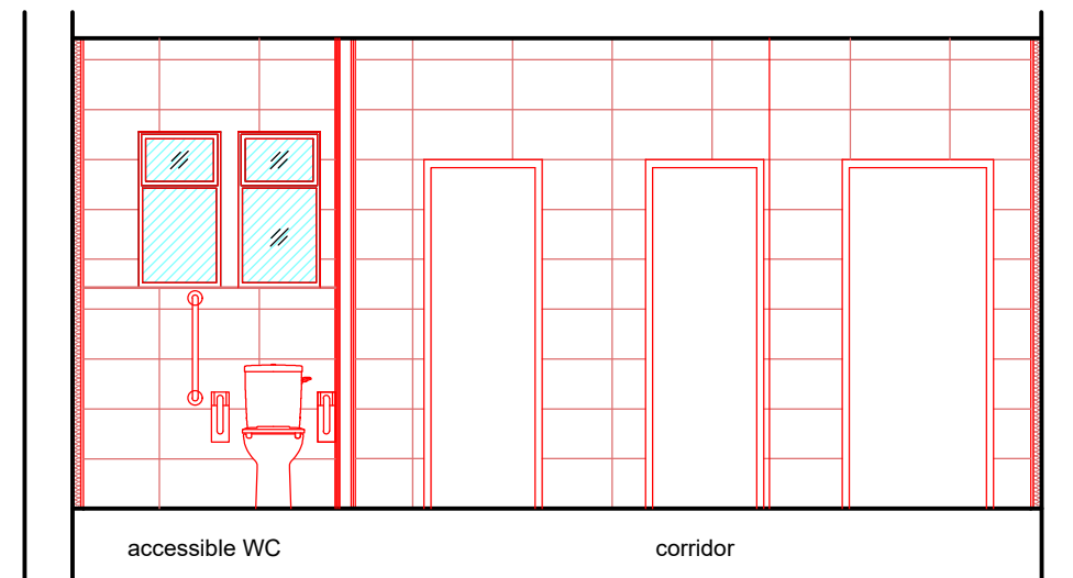
WC corridor wall east facing elevation as proposed 1:50
