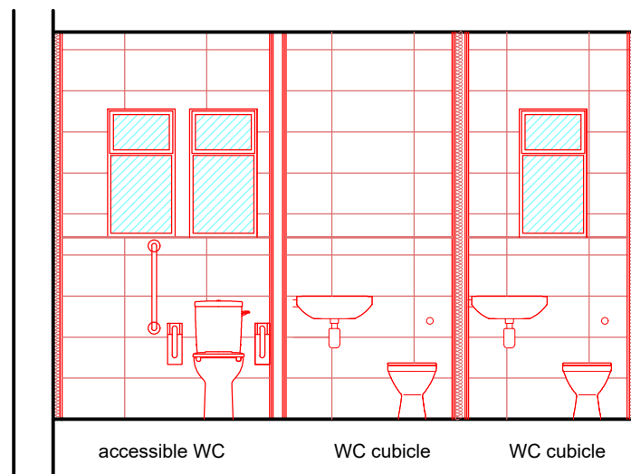
WC cubicles east facing elevation as proposed 1:50
