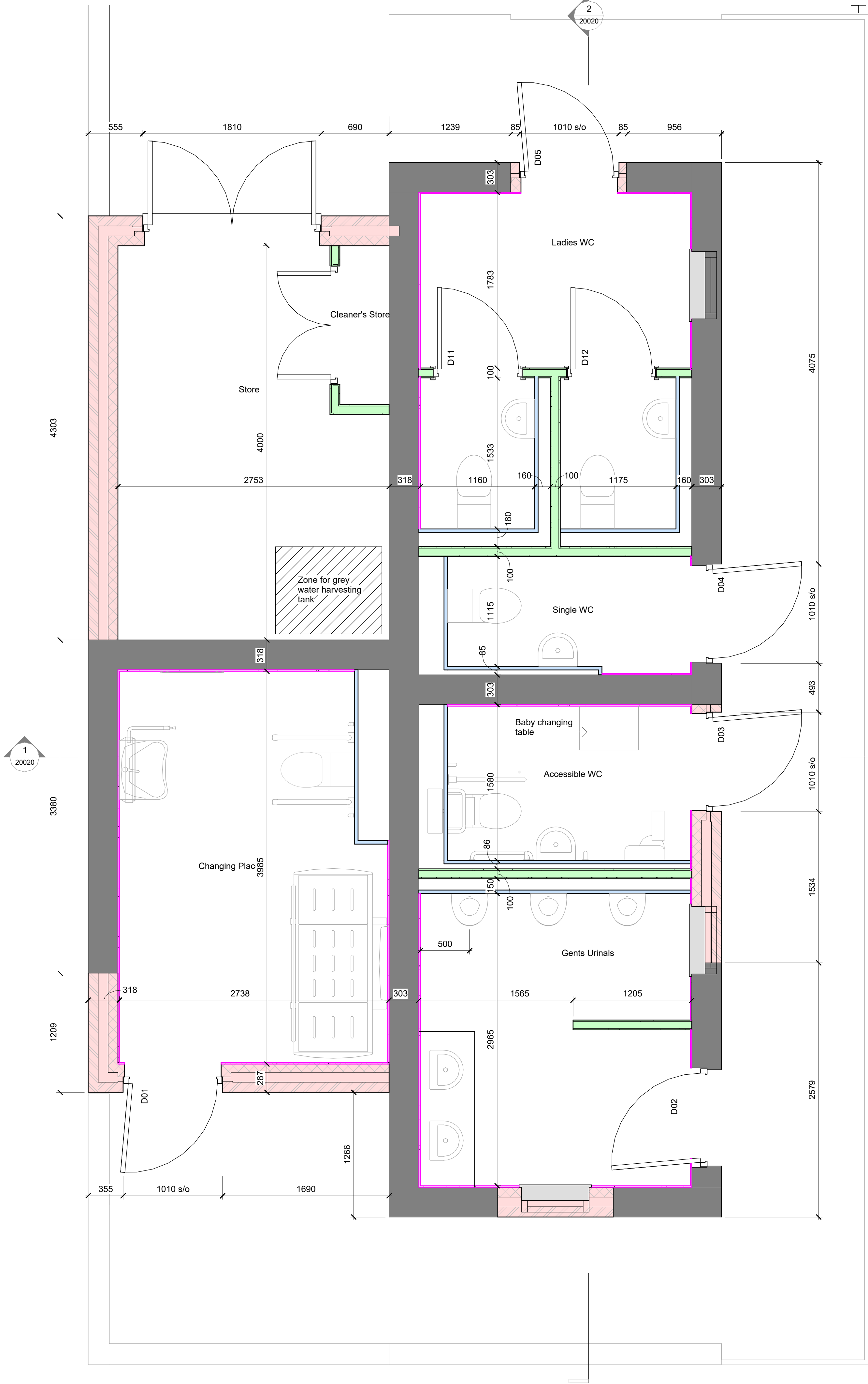
Toilet Block Plan - Proposed
