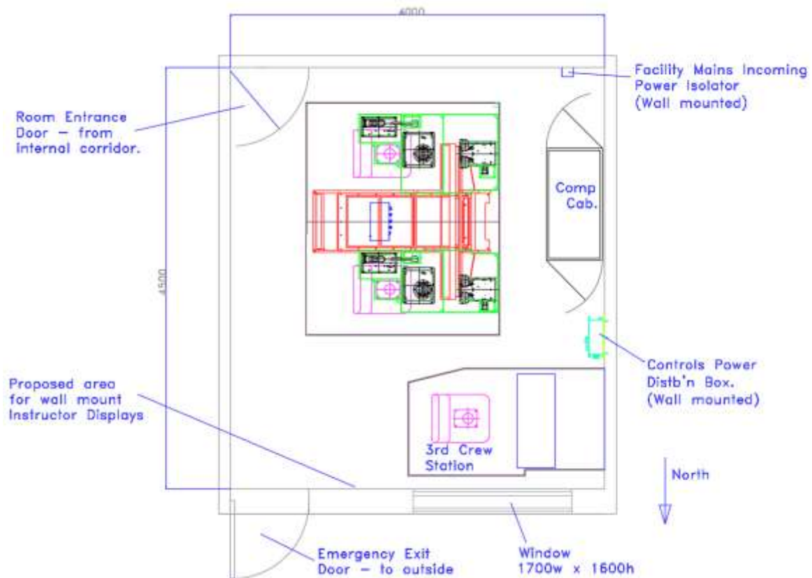
Figure 2 - Plan view of FPT layout at RAF Benson
