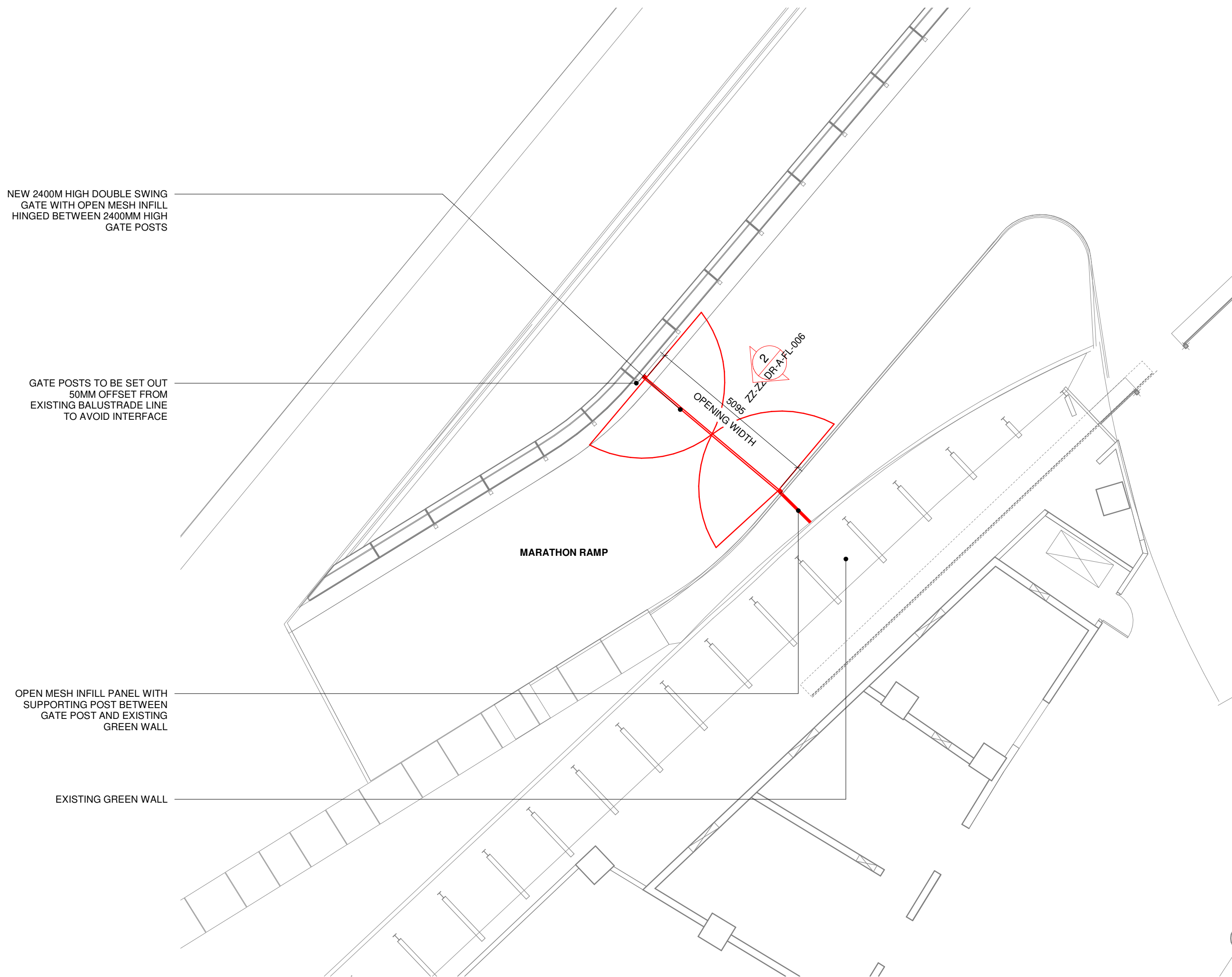
1 PLAN MARATHON RAMP GATE SETTING OUT PLAN 1 : 100
