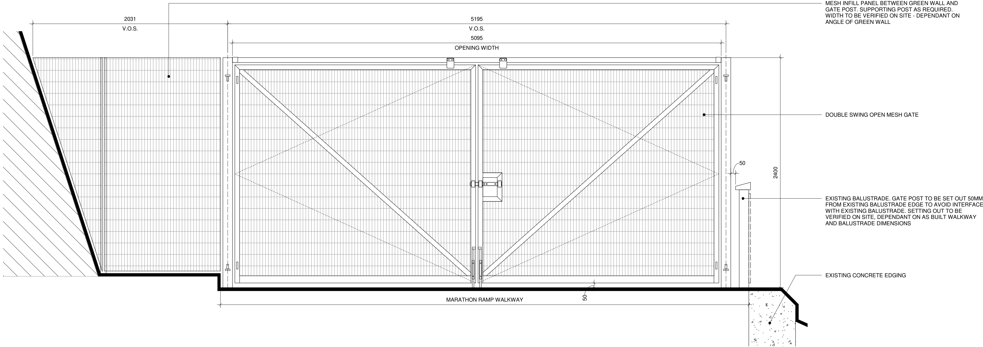
2 ELEVATION MARATHON RAMP GATE SETTING OUT ELEVATION 1 : 20
