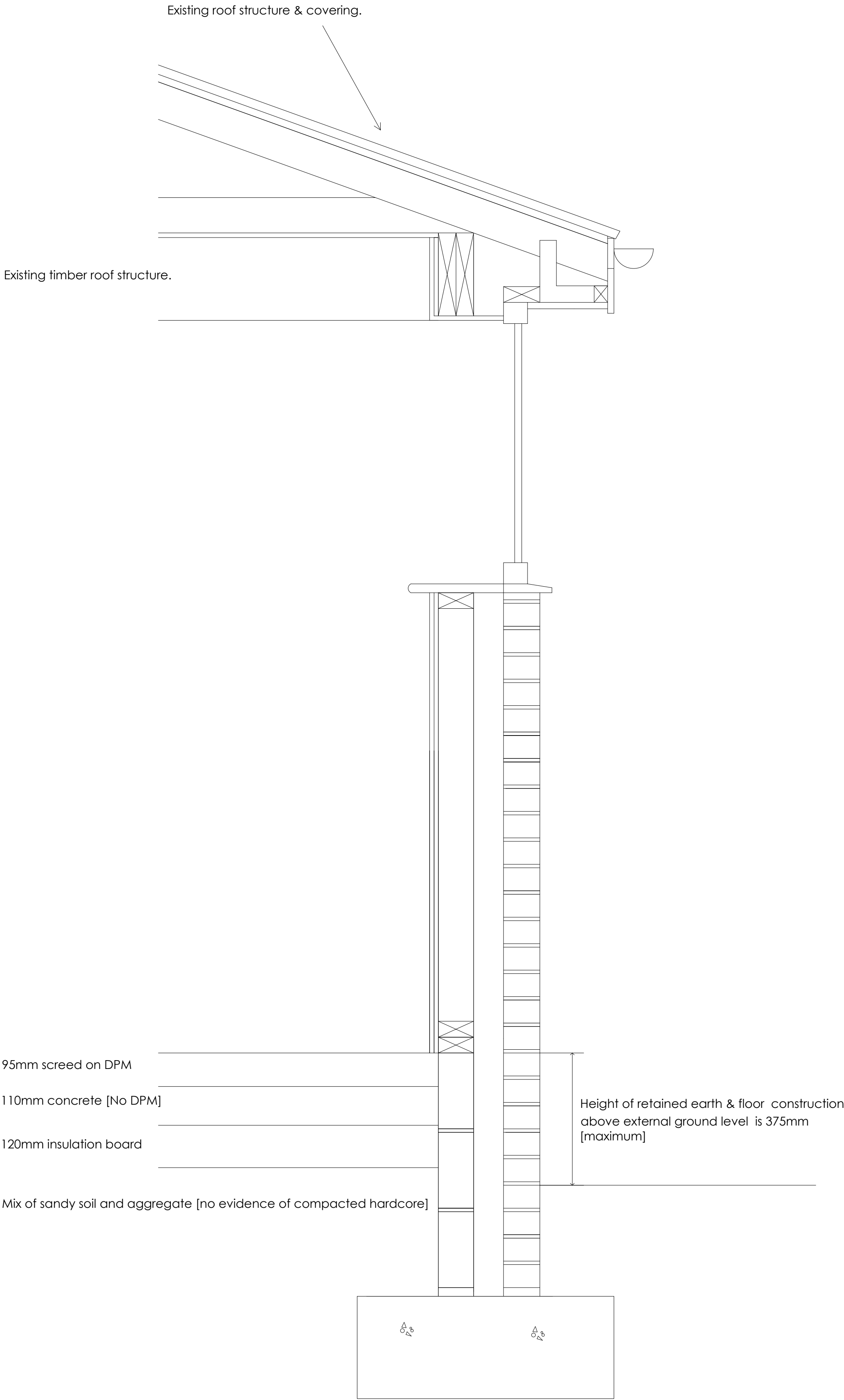
EXISTING SECTION A-A [OFFICE]
