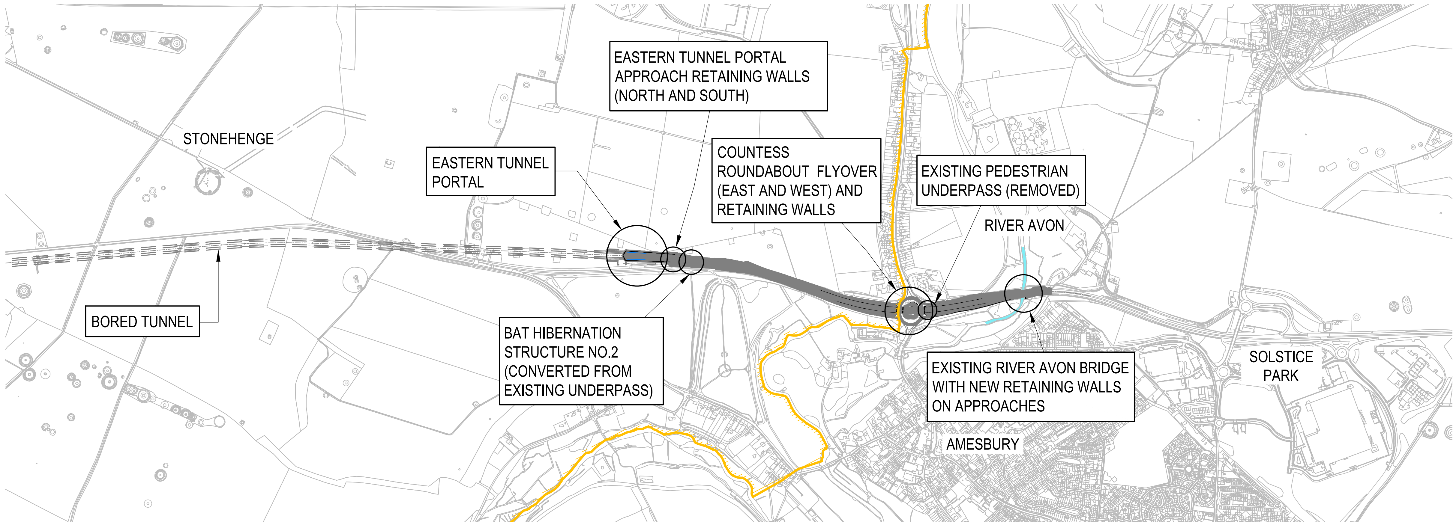
STRUCTURES LOCATION PLAN (CONTINUED) SCALE 1:10000
