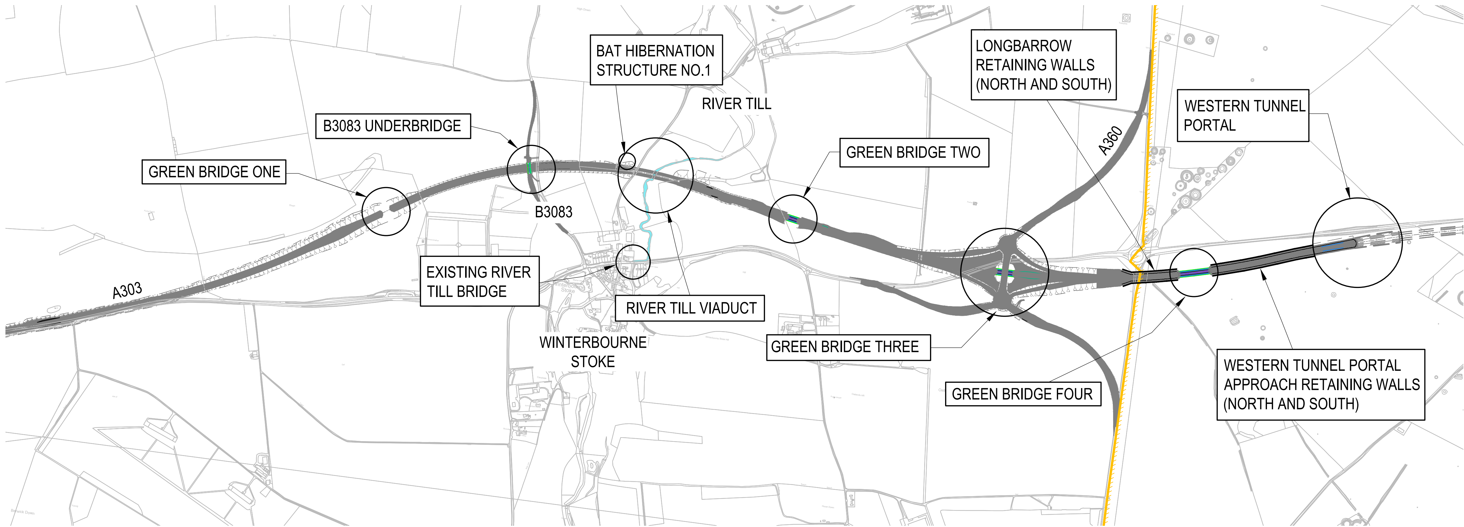
STRUCTURES LOCATION PLAN SCALE 1:10000
