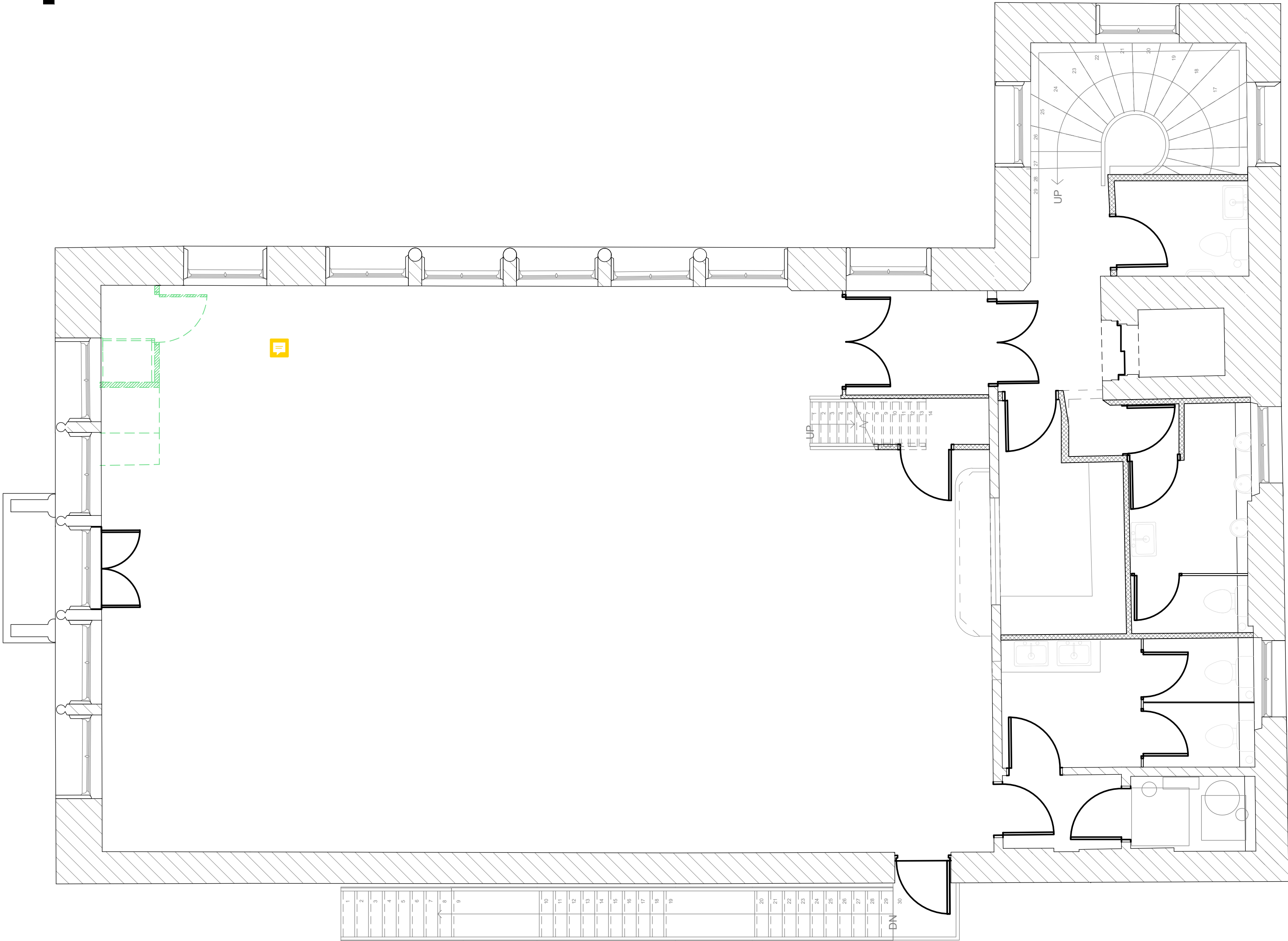
PROPOSED SECOND FLOOR REMOVAL/ DEMOLITION PLAN - scale 1:50
