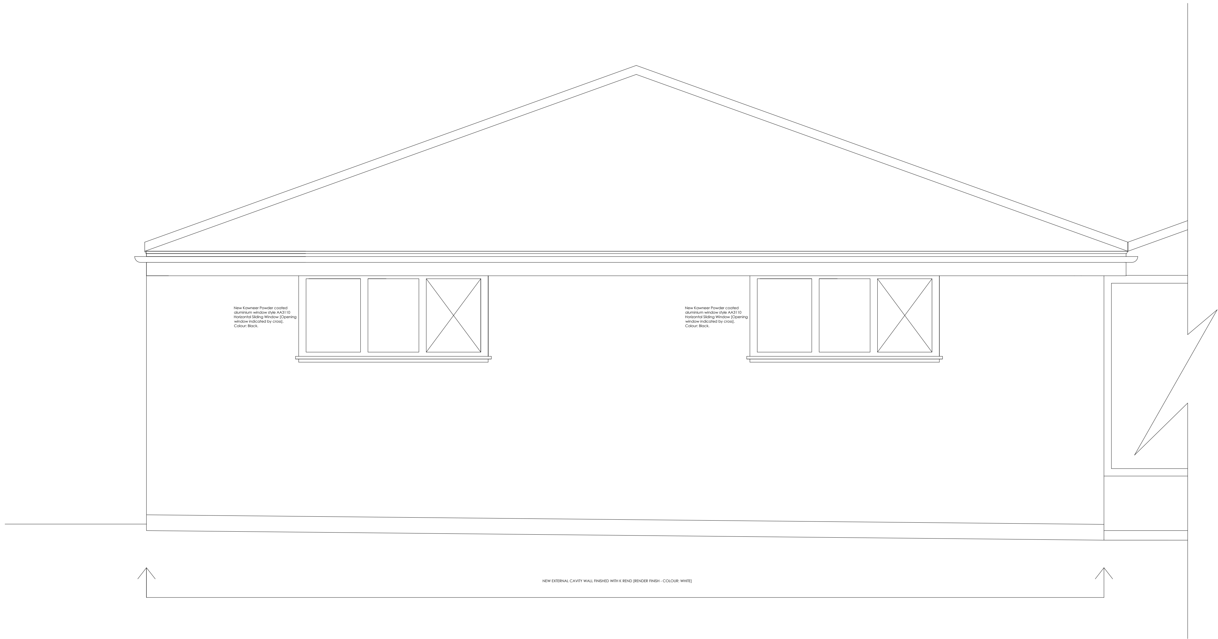
PROPOSED FRONT [NORTHERN] ELEVATION - OFFICE - DRAWING HAR006
