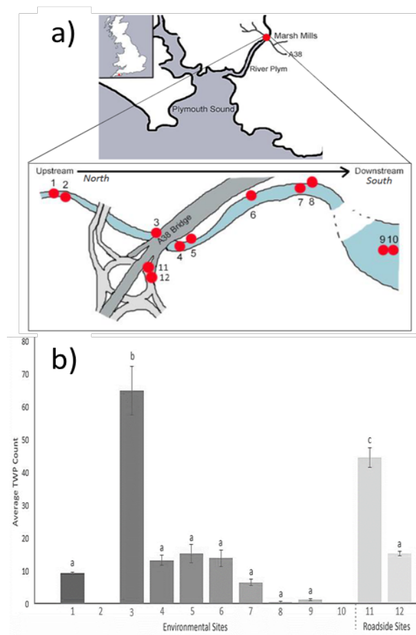
Figure 3a) Sketch map indicating sampling locations in the vicinity of the A38 trunk road near to Plymouth; b) abundance of tyre particles (Mean \pm SE) at each location based on visual characteristics. Locations with the differing letters of the alphabet were statistically different.
