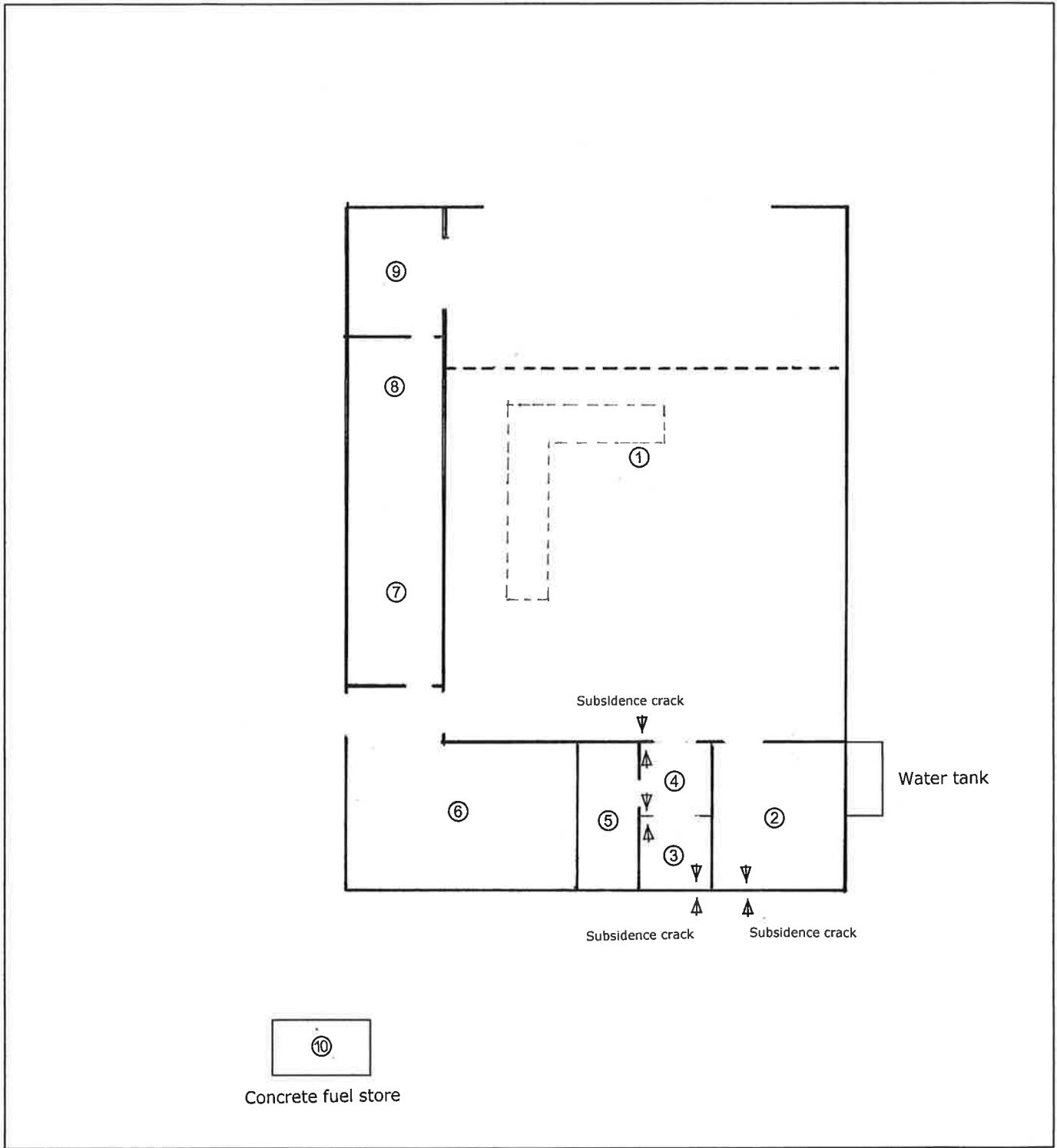
Willett Hill Depot layout Not to scale
