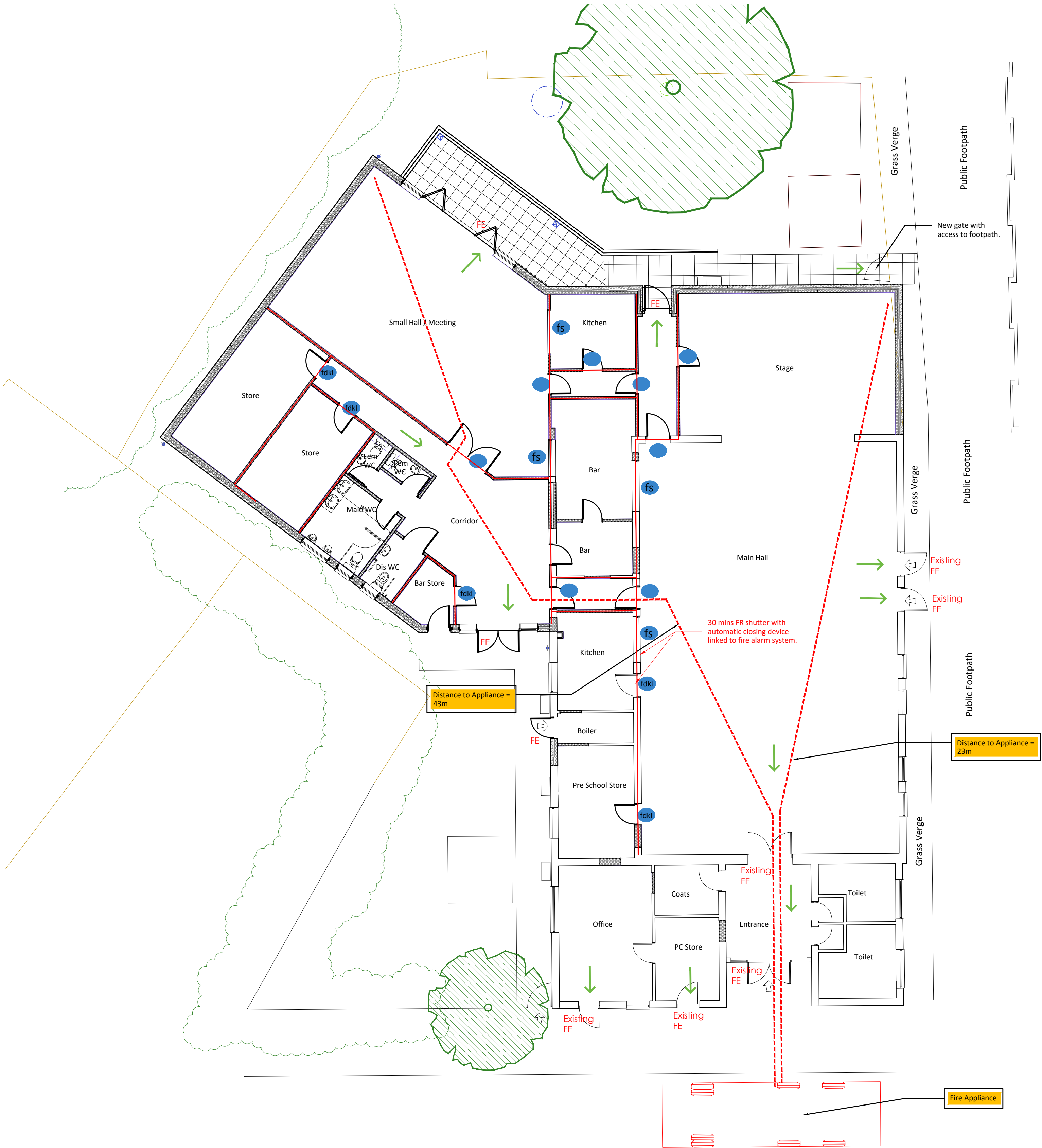
Ground Floor Plan / Fire Strategy As Proposed
