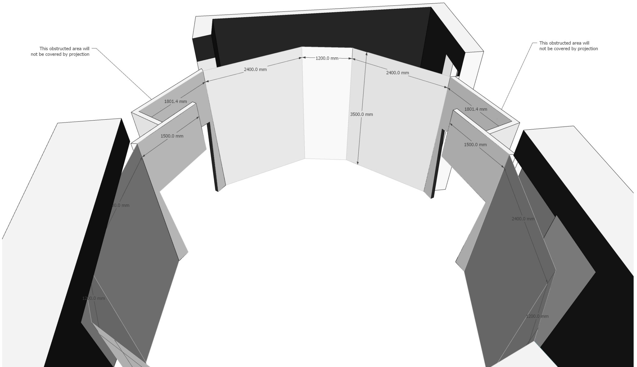
Immersive AV System – Appendix H Projection Map Coverage
