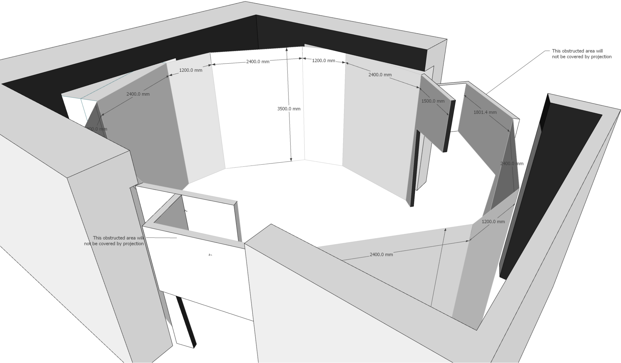
Model with dimensions (3)
