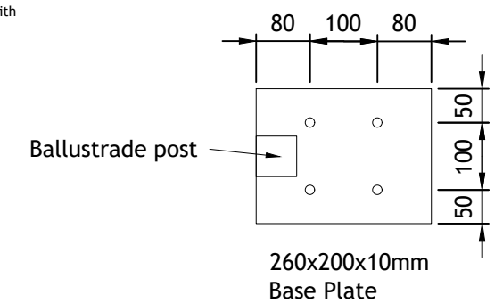
Detail 4 1:5
