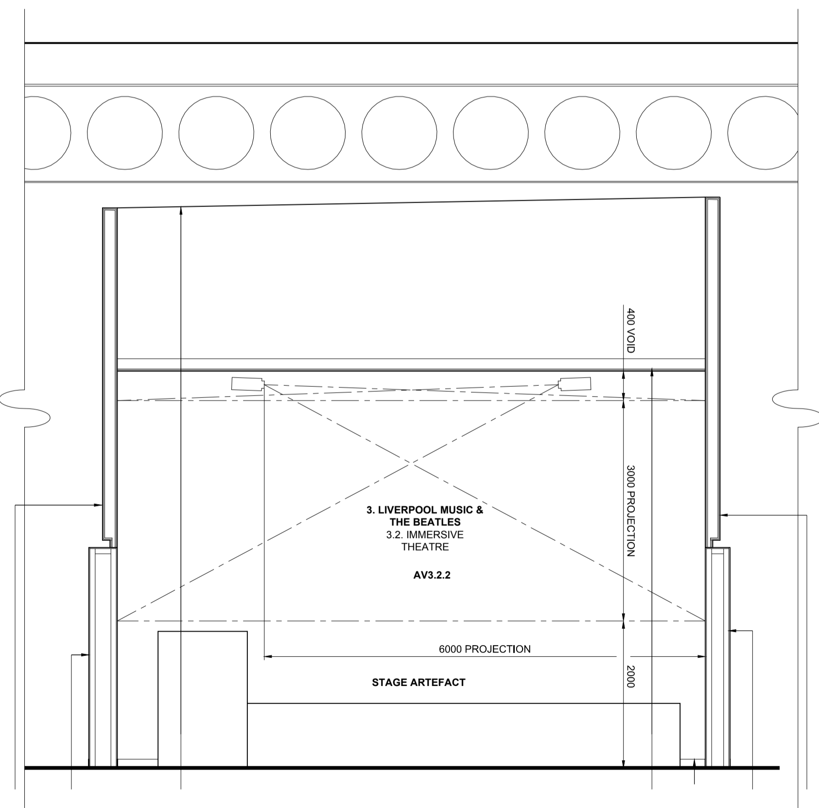
3 AREA 3.0 MUSIC & THE BEATLES ELEVATIONS Scale 1:50
