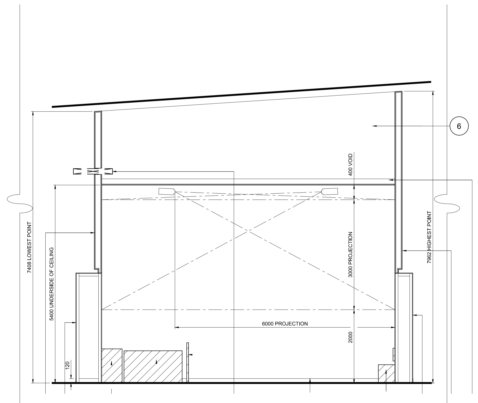
4 AREA 3.0 MUSIC & THE BEATLES ELEVATIONS Scale 1:50
