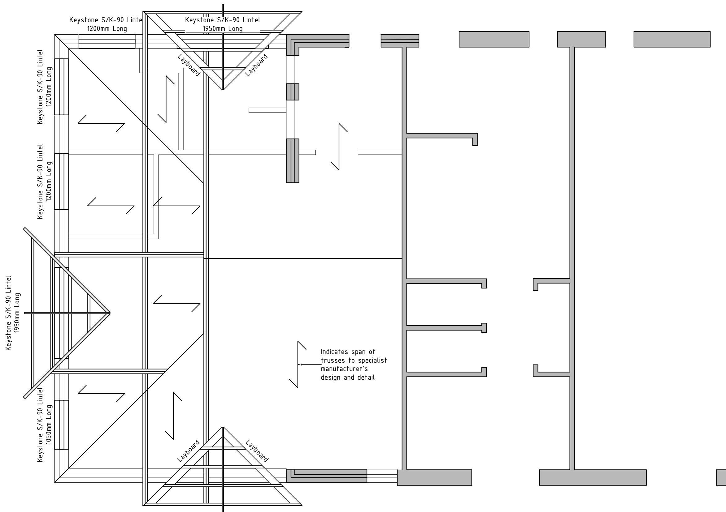
Roof Structure Layout 1:50
