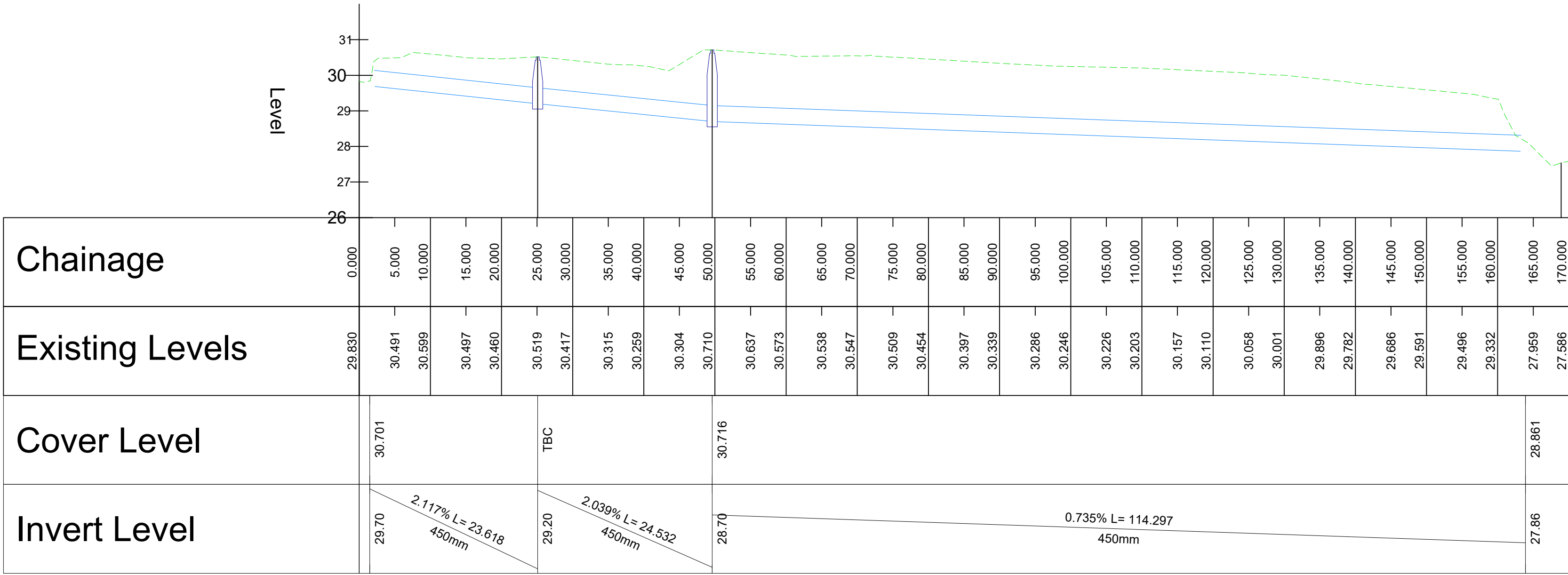
PIPE ALIGNMENT - LONGSECTION CHG. 0-170 SCALE: H 1:500,V 1:100. DATUM: 26.000
