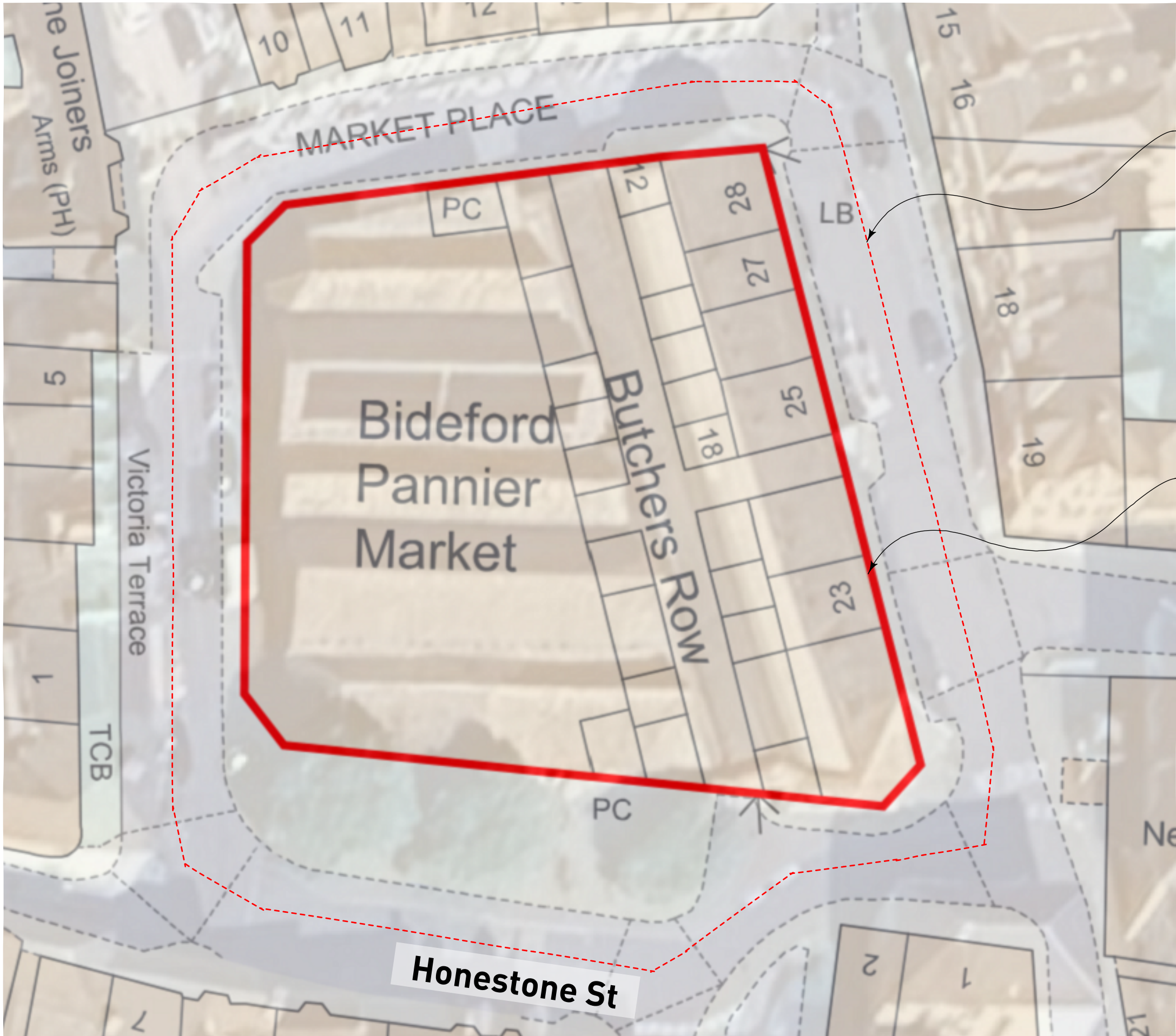
SITE PLAN SHOWING TOPOGRAPHIC SURVEY EXTENTS
