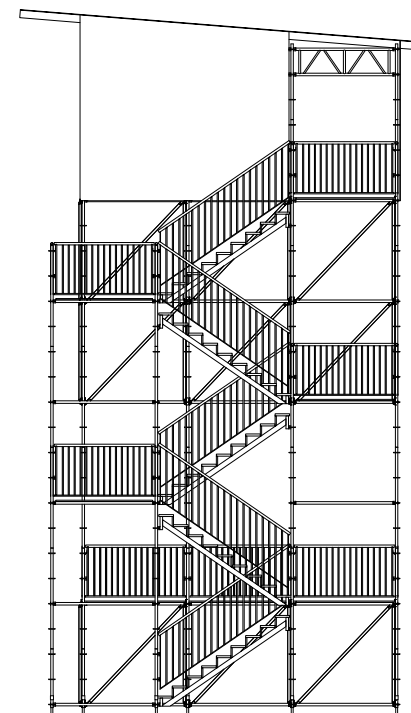
SIDE ELEVATION
