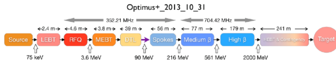
Figure 1-1 : Schematic of ESS Linac
