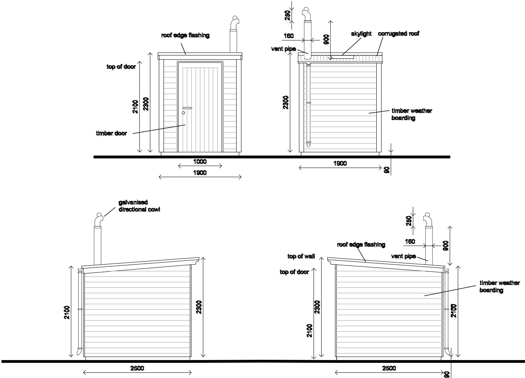
Composting Toilet Elevations
