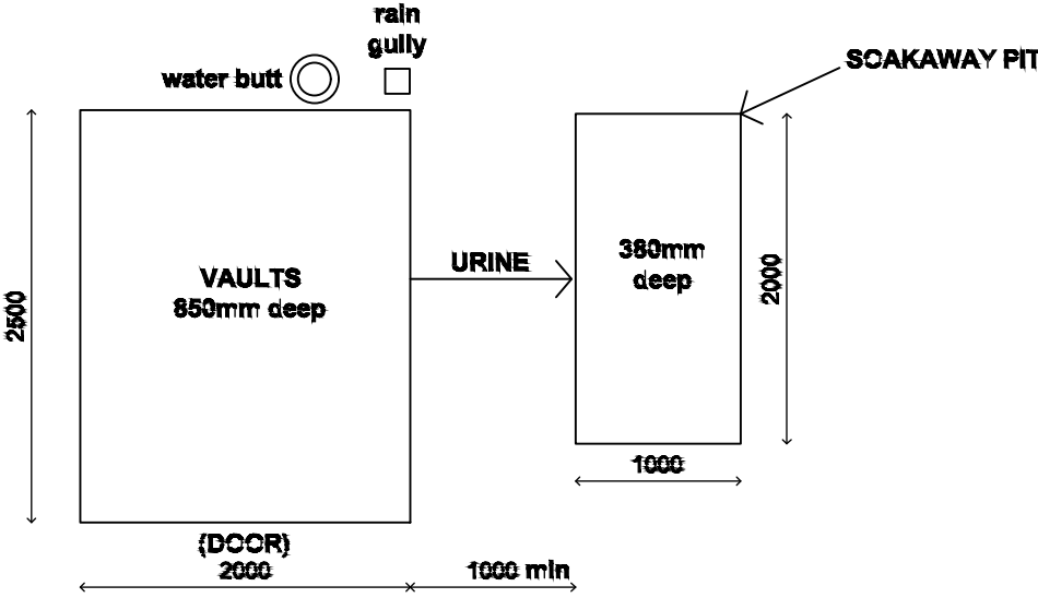
Composting Toilet Detail
