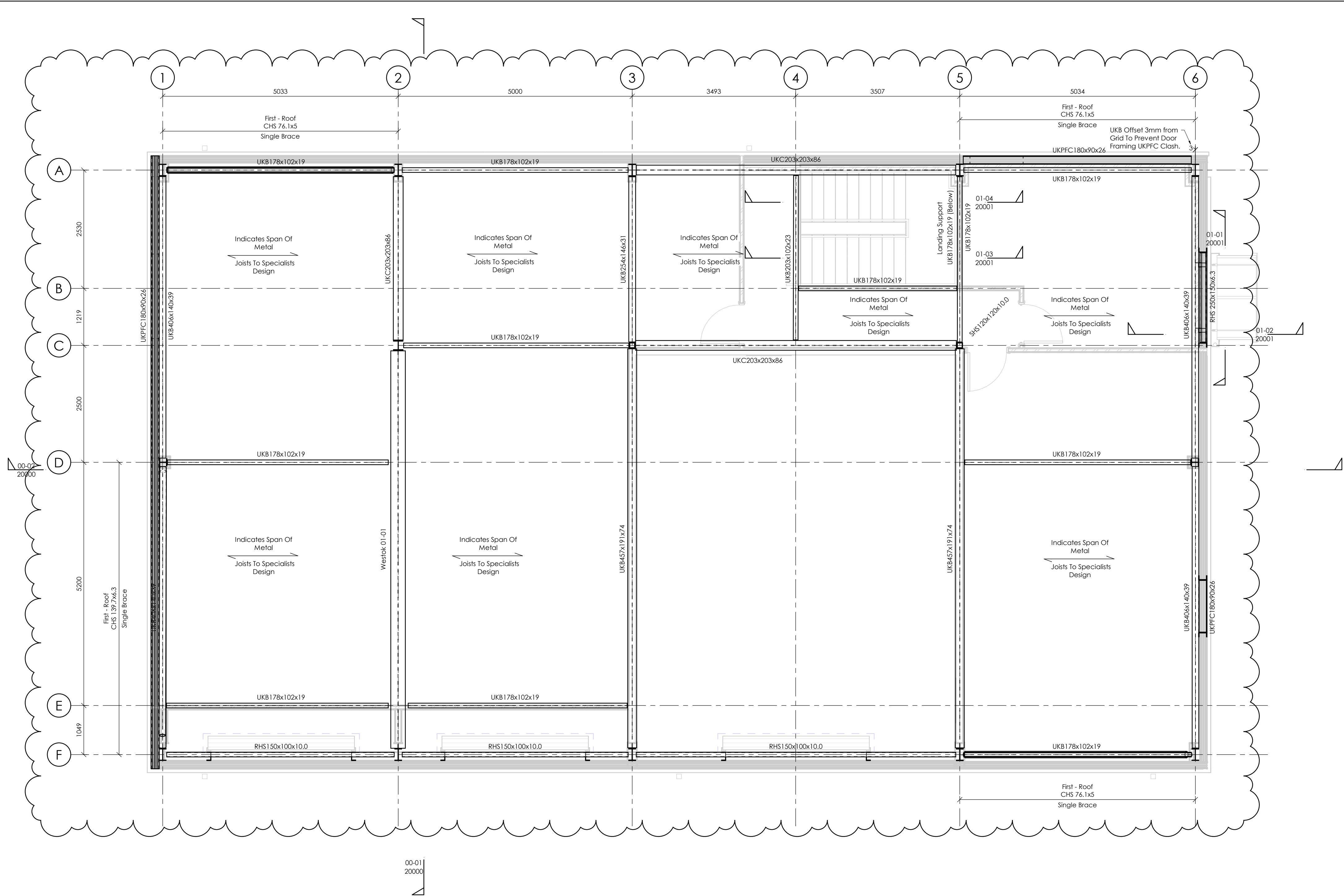
FIRST FLOOR STRUCTURE LAYOUT
