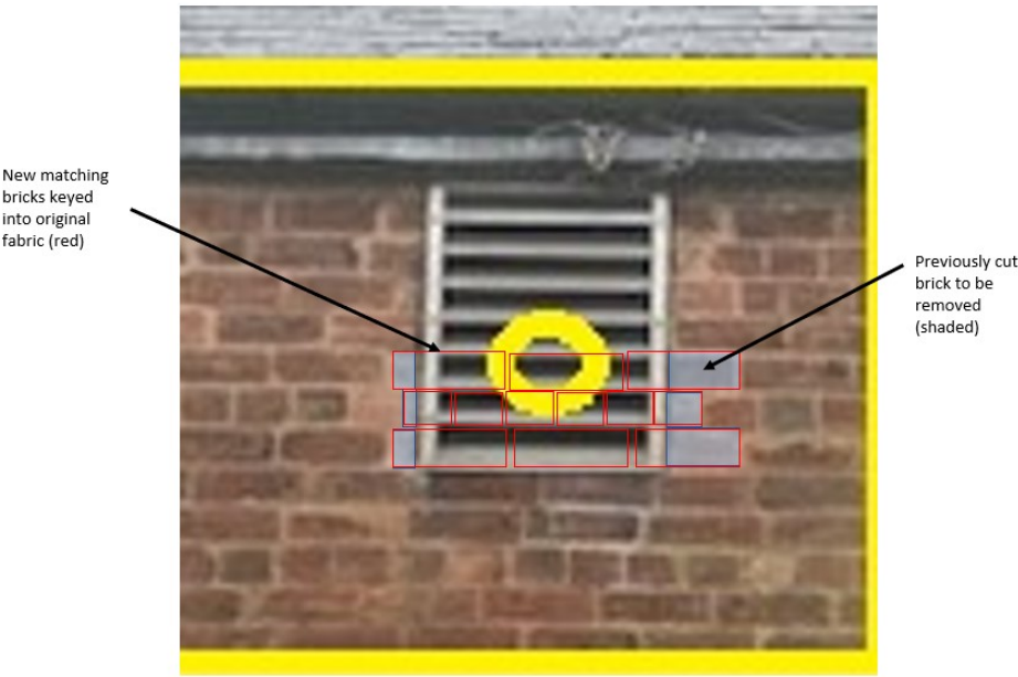
Figure 2: Brick work infill requirements
