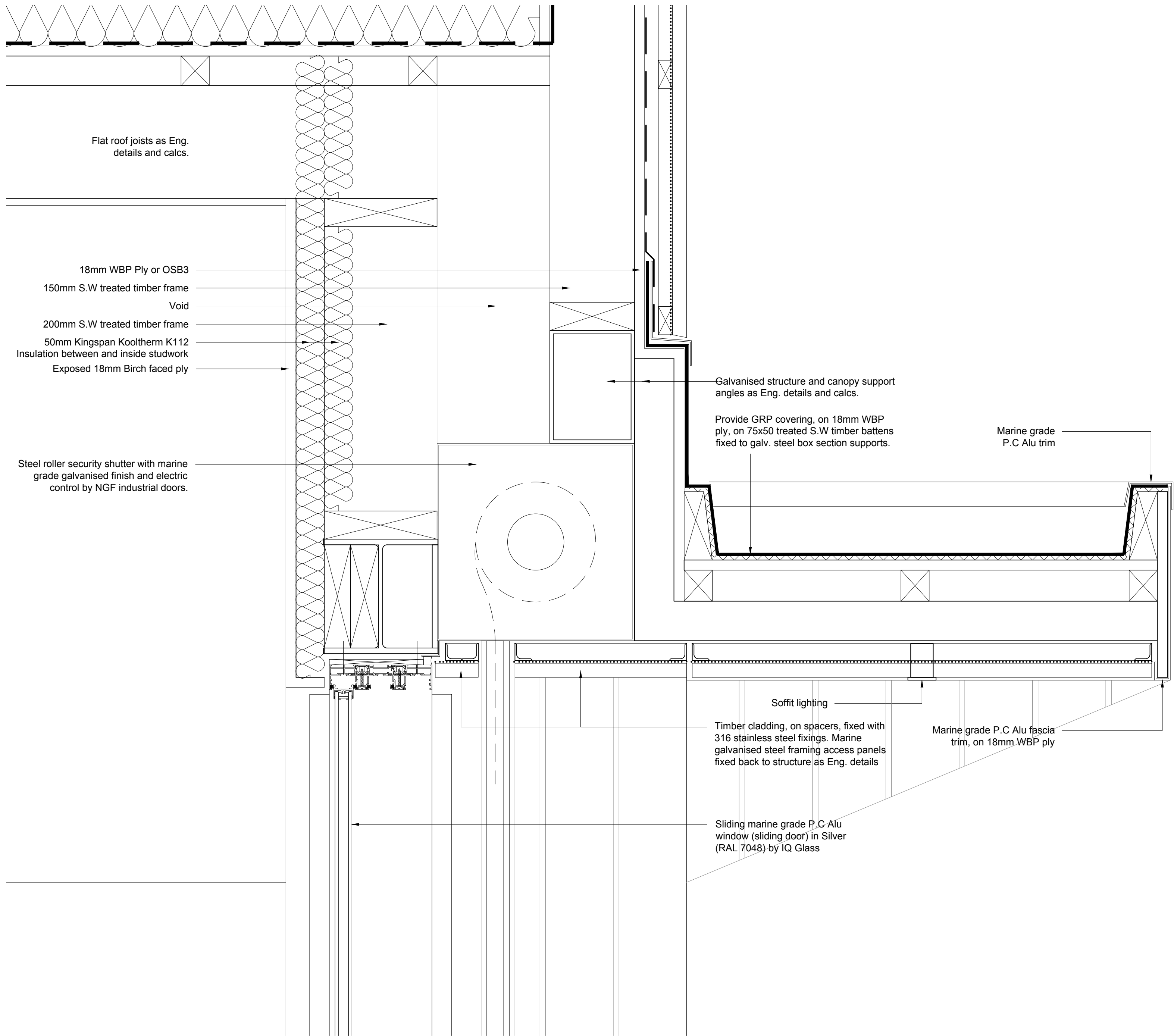
Sliding door head / shutter detail 1:5
