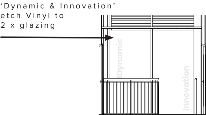
2 F01 - Elevation 1 Scale 1 : 50
