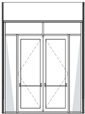
3 G01 - Elevation 2 Scale 1: 50
