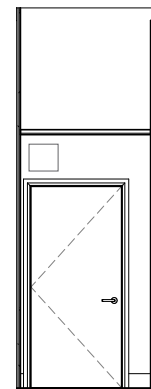
15 G08 - Elevation 4 Scale 1 : 50
