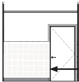
3 F06 - Elevation 2 Scale 1 : 50
