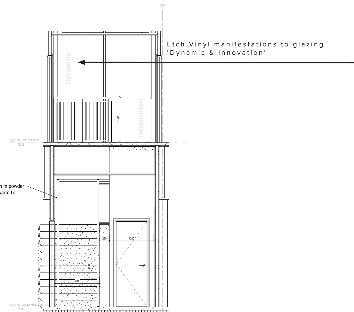
2 Cross Section Through Stair Scale 1 : 20
