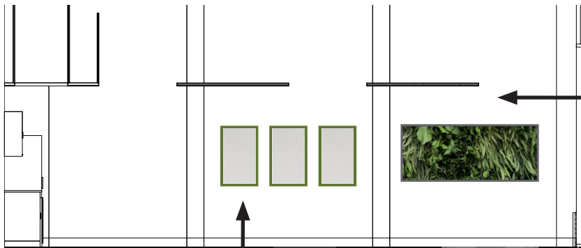
2 G02 - Elevation 3 Scale 1 : 50
