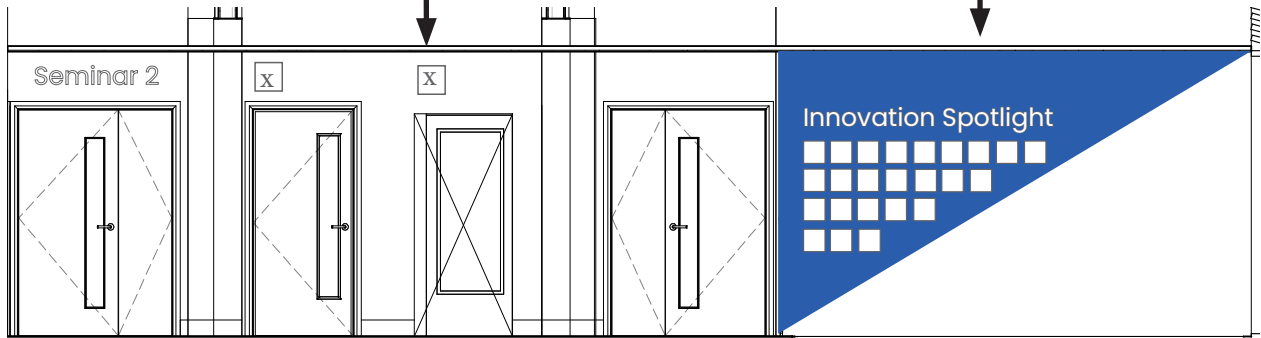
5 F01 - Elevation 4 Scale 1 : 50
