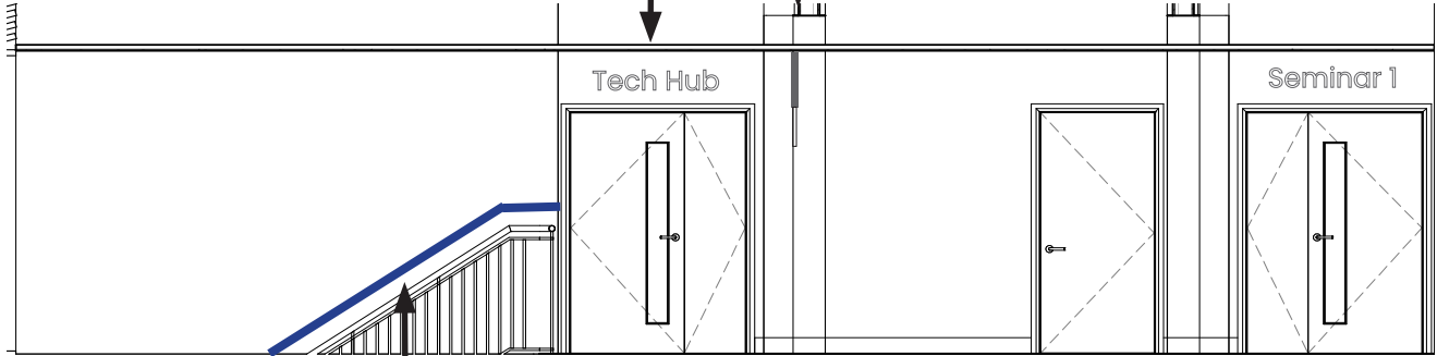
3 F01 - Elevation 2 Scale 1 : 50
