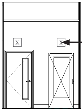
5 G01 - Elevation 4 Scale 1: 50
