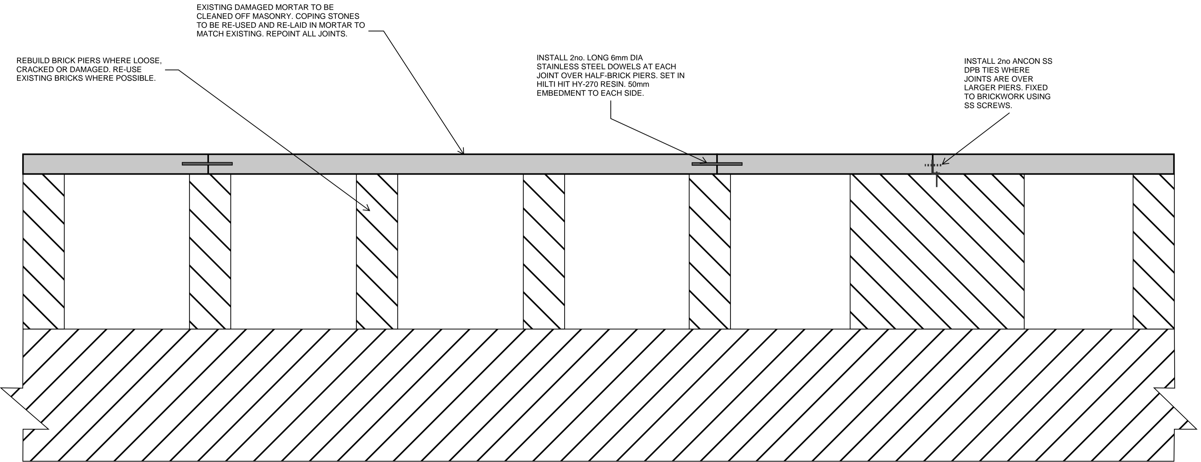
LOOSE COPING STONES ON ACCESSIBLE PIERED MASONRY WALL - TYPICAL REPAIR DETAIL
