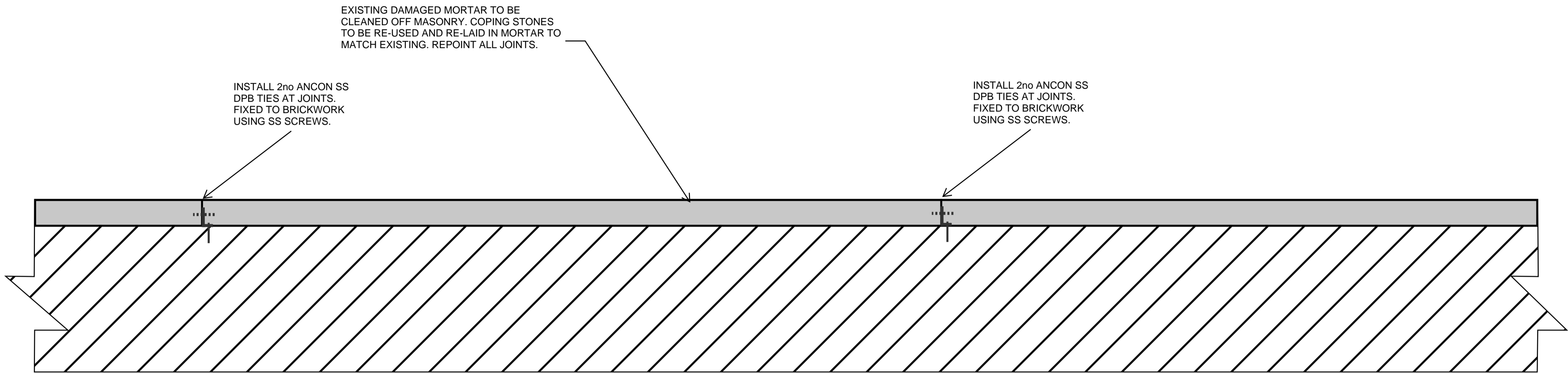
LOOSE COPING STONES ON ACCESSIBLE SOLID MASONRY WALL - TYPICAL REPAIR DETAIL
