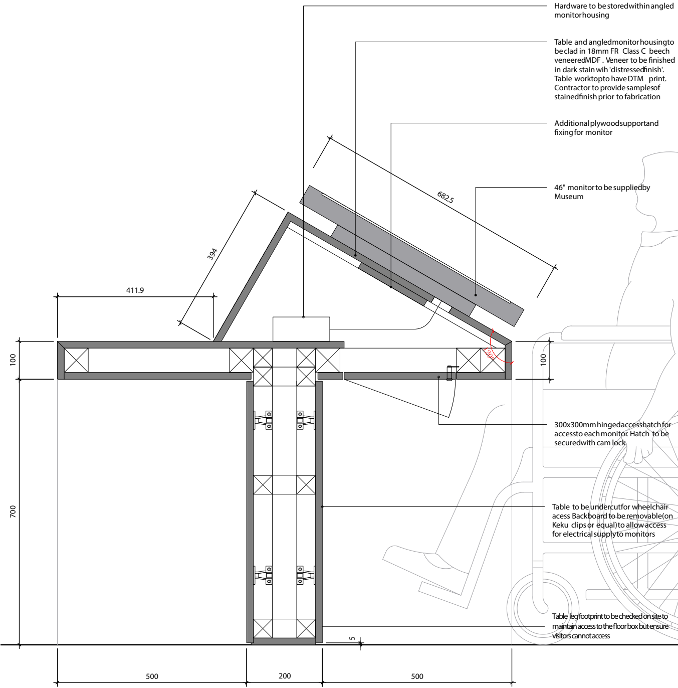
03 SB07 Section Detail (1:10 at A3)
