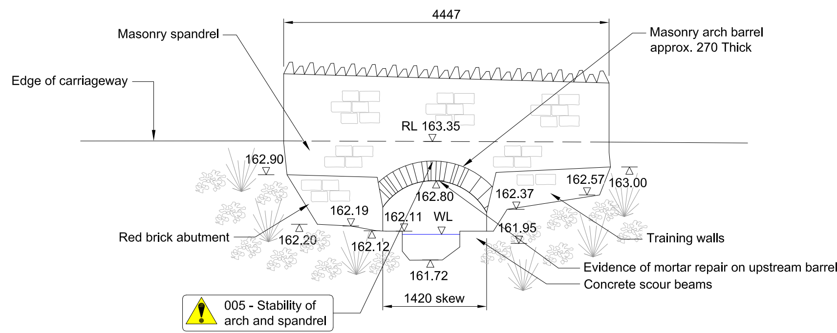
Upstream Elevation 1:50
