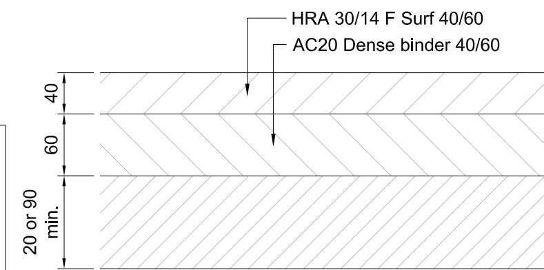
Surfacing Detail (interface with existing) 1:5
