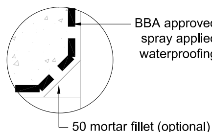
Detail 3 1:5
