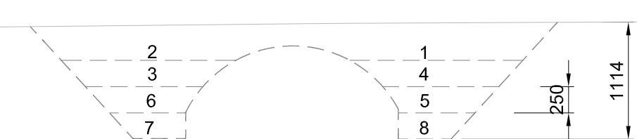
Sequence of Excavation (Balanced Excavation) 1:50
