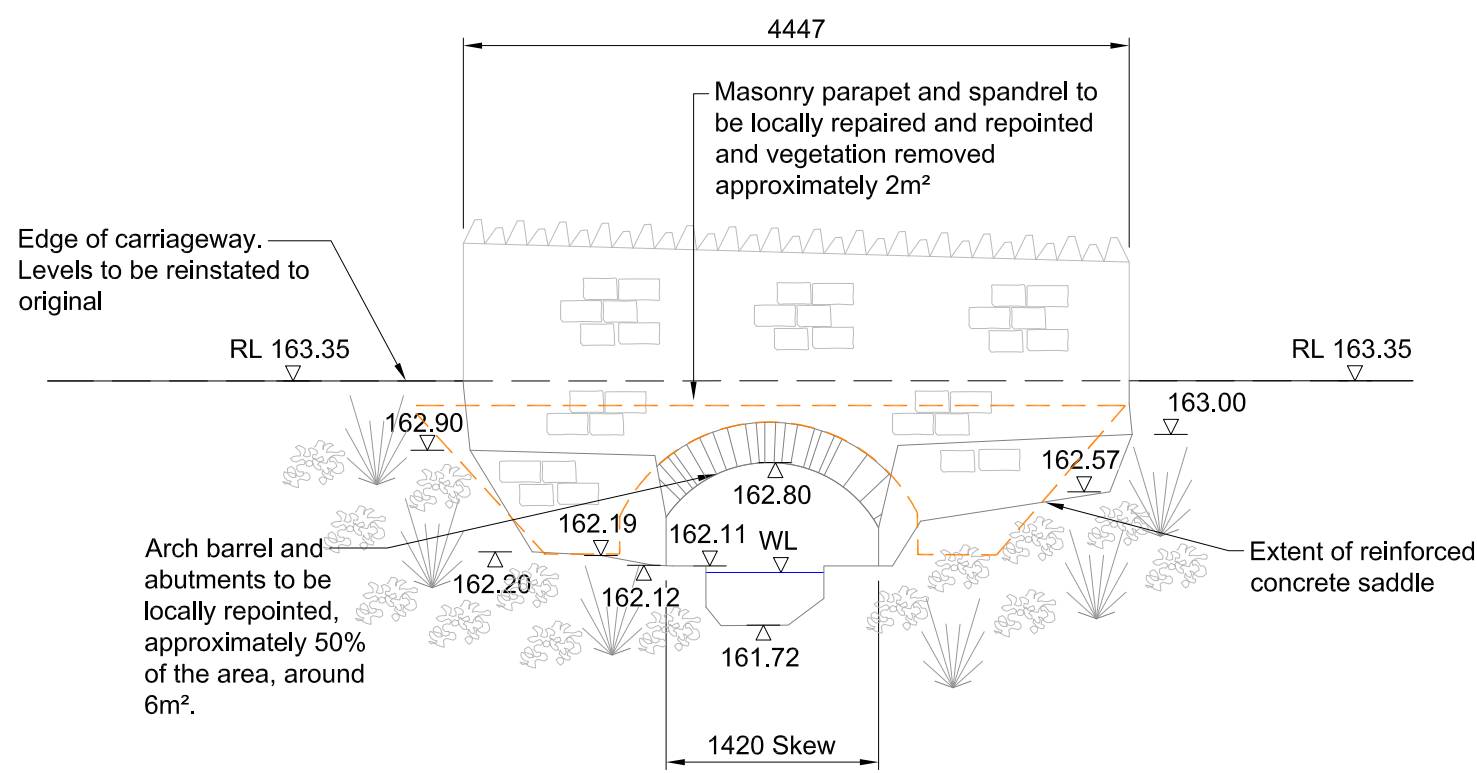
Upstream Elevation 1:50
