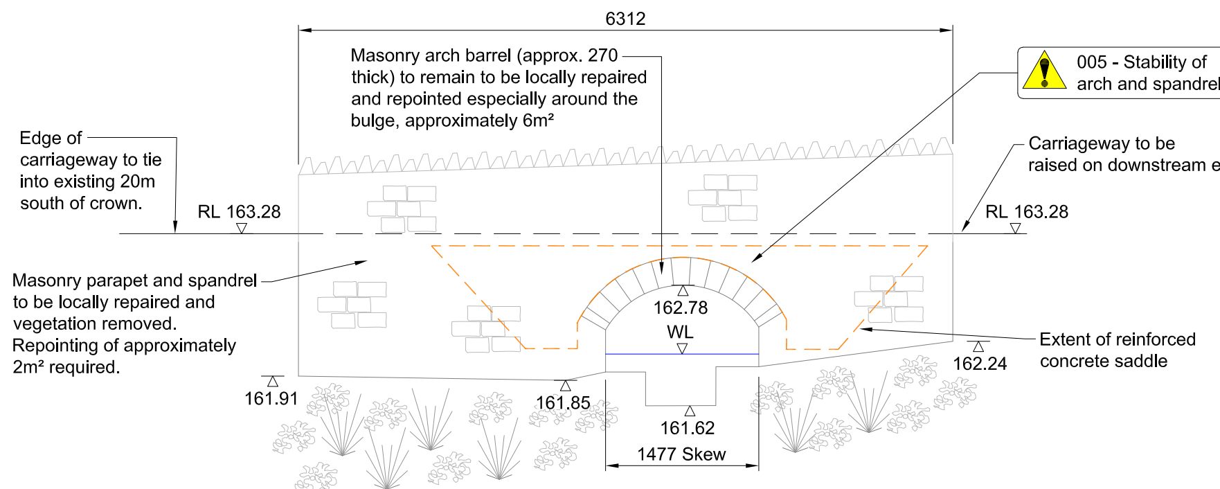
Upstream Elevation 1:50
