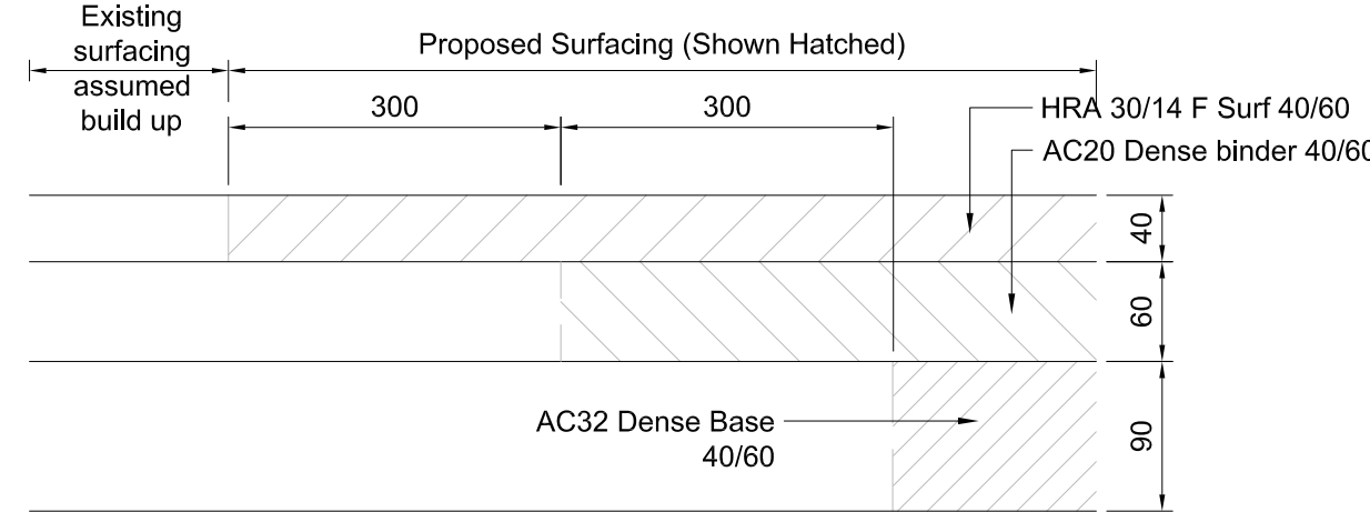
Surfacing Detail (interface with existing) 1:5
