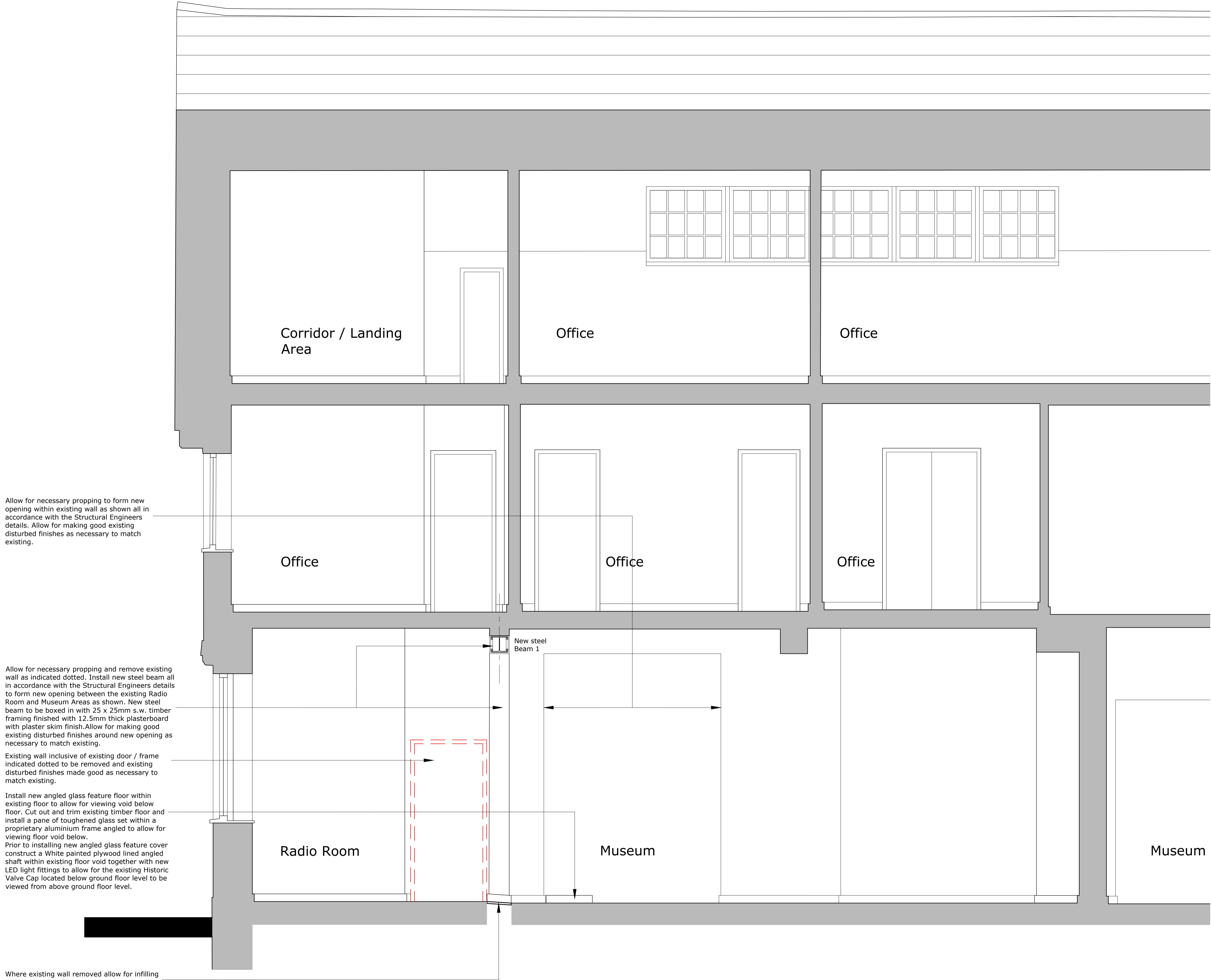
Section C-C Through Existing
