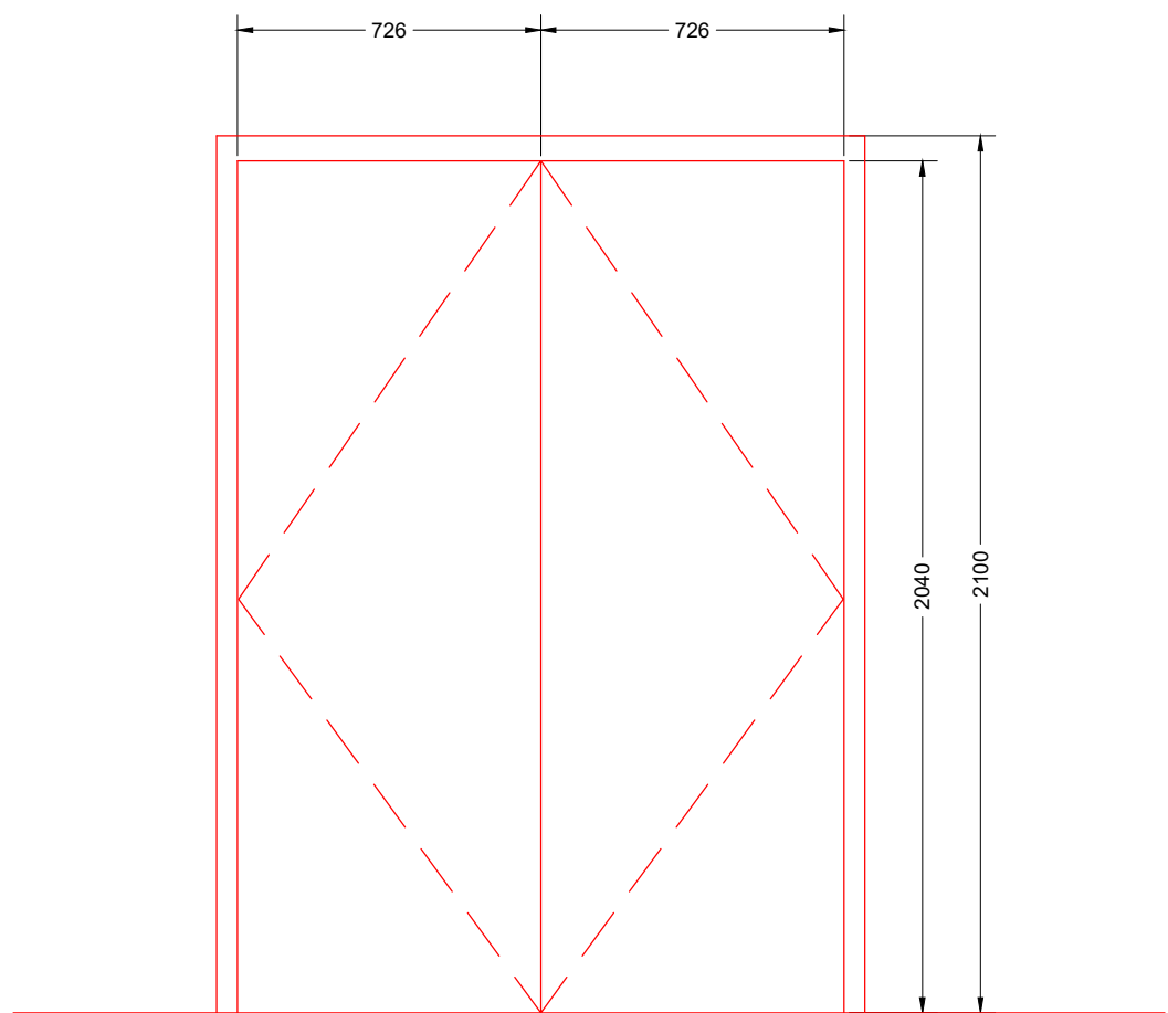
Door Type I Door D24 (cleaners cupboard)
