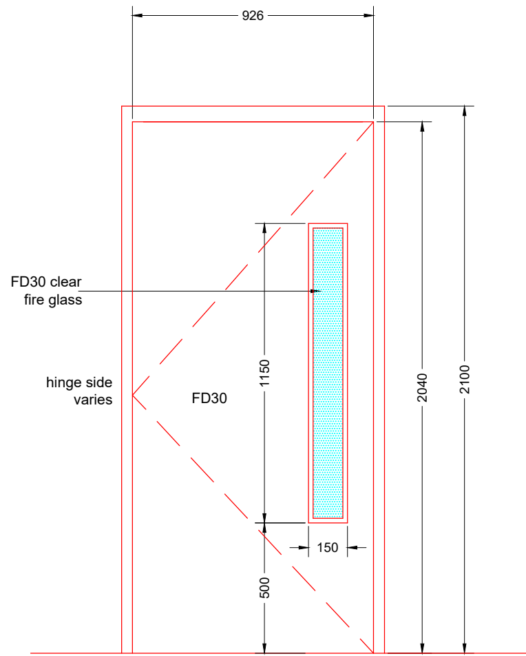
Door Type C Doors D7 & D8 (switch room and store)
