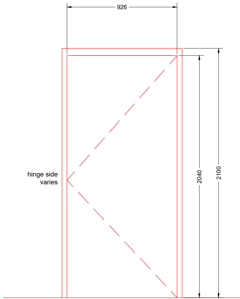
Door Type B Doors D2, D6 (accessible WC's)
