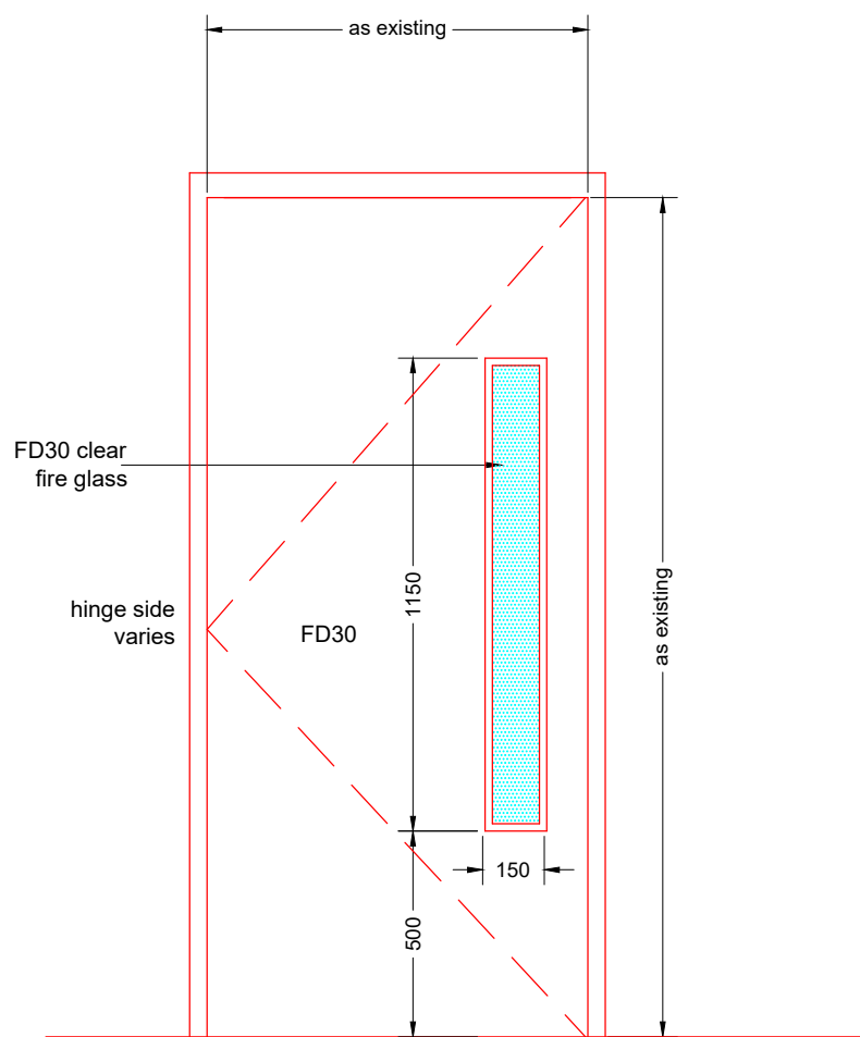
Door Type J Door D25 (reception)
