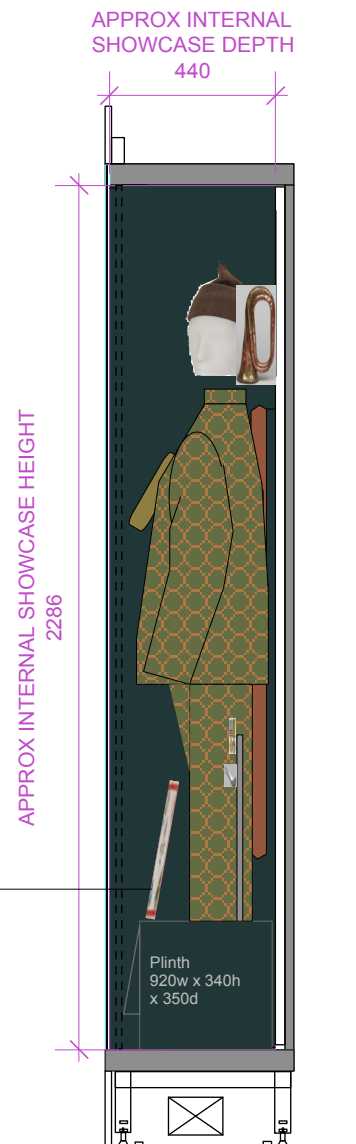
Side elevation
