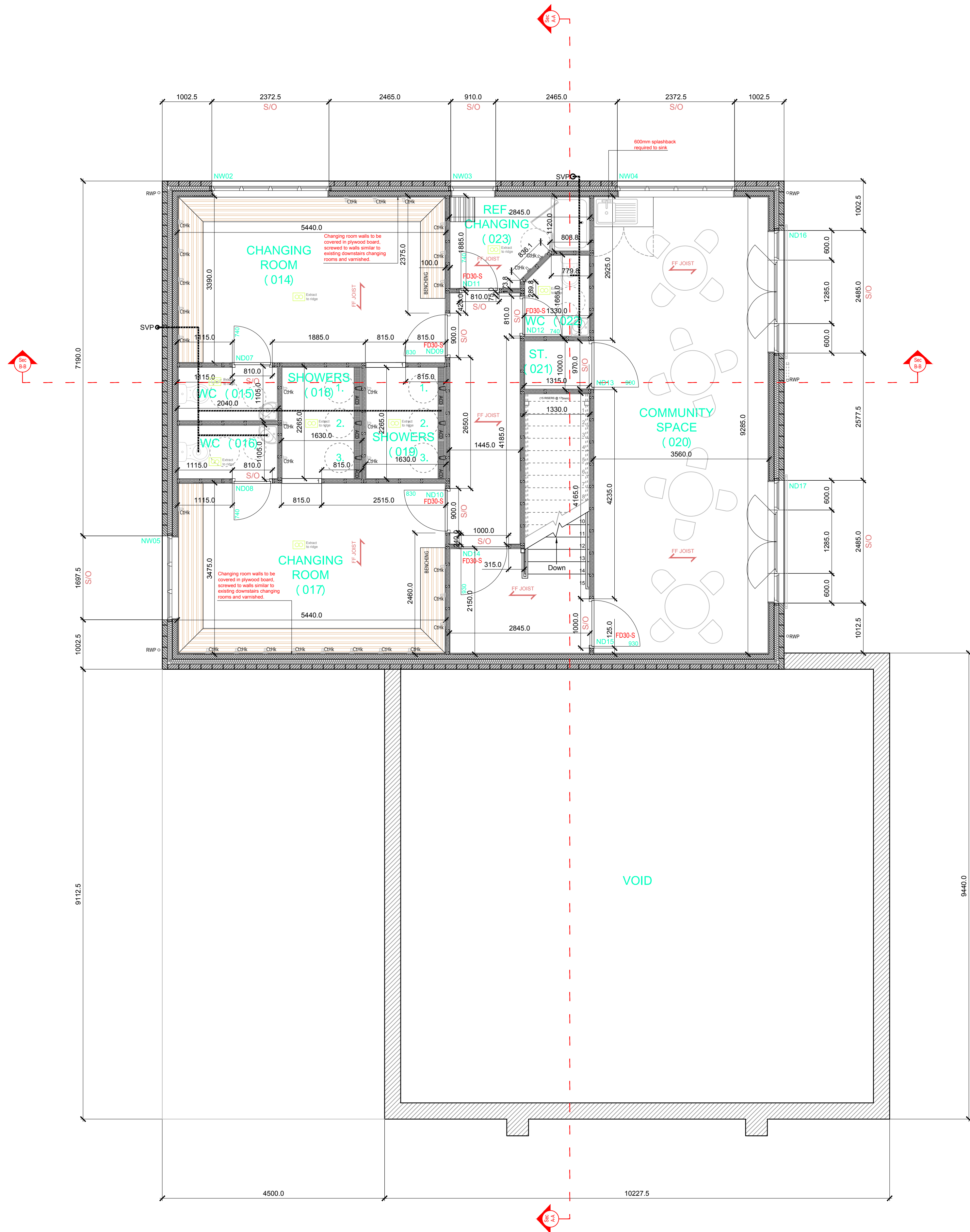
FIRST FLOOR PLAN, SCALE: 1:50 @ A1
