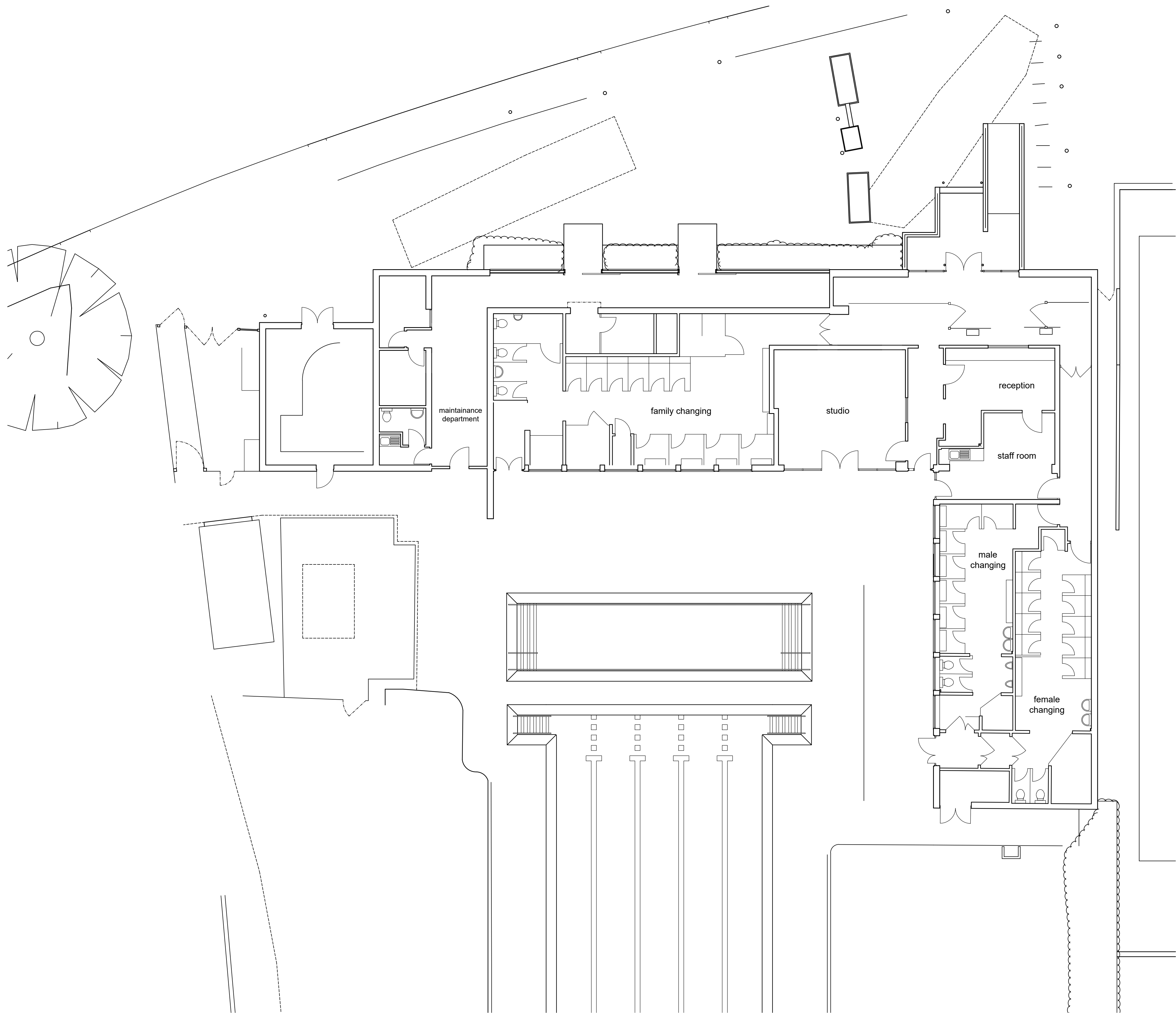
ground floor plan as existing 1 : 100
