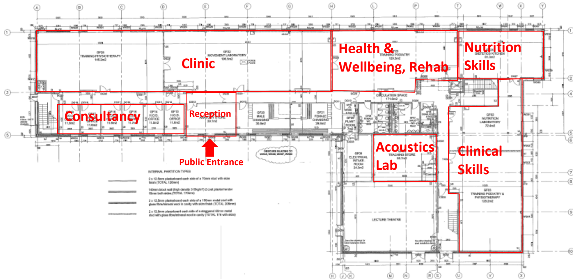
Building – Ground Floor Layout (highlighting potential areas of reconfiguration)
