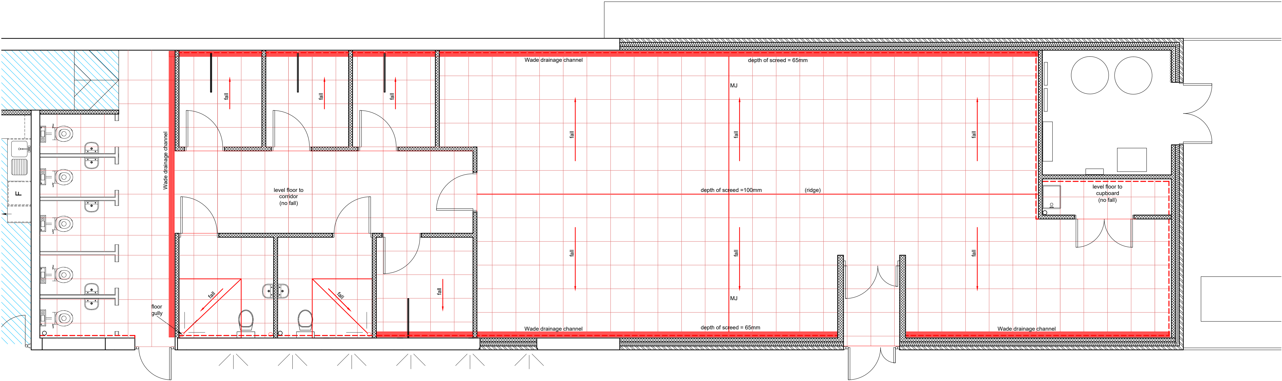
changing room floor finishes as proposed 1 : 50
