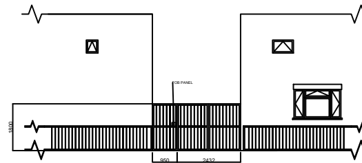
PROPOSED FRONT ELEVATION 32 BLENHEIM CRESCENT VIEW
