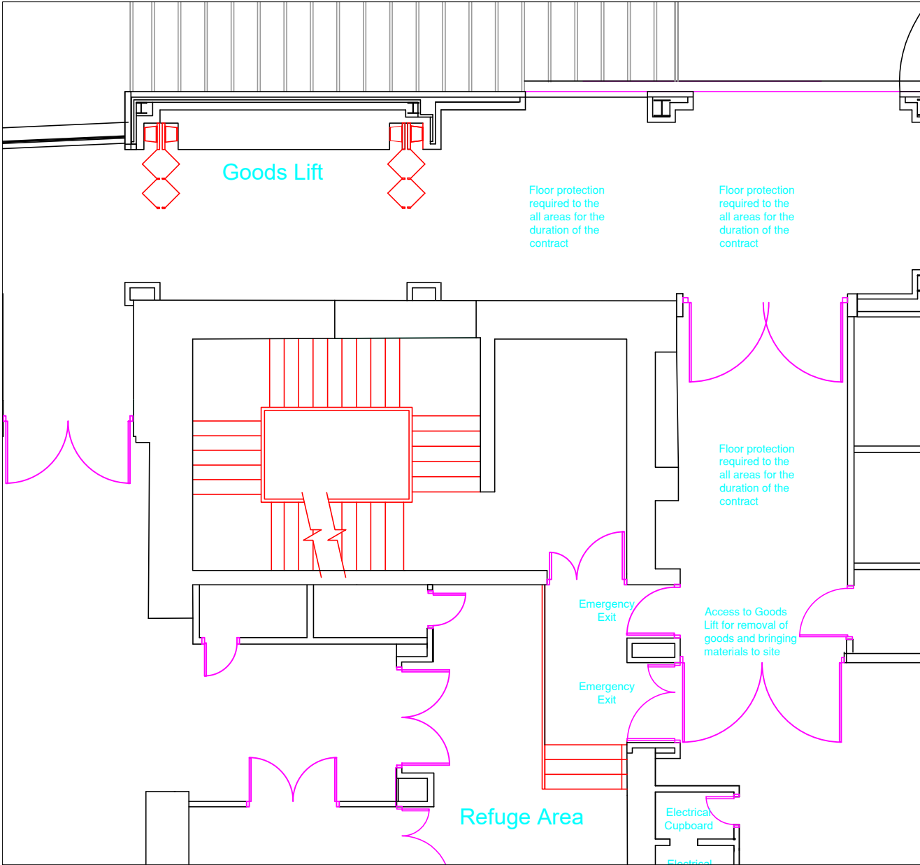
Third Floor Goods Entrance and Stairwell- 1/100
