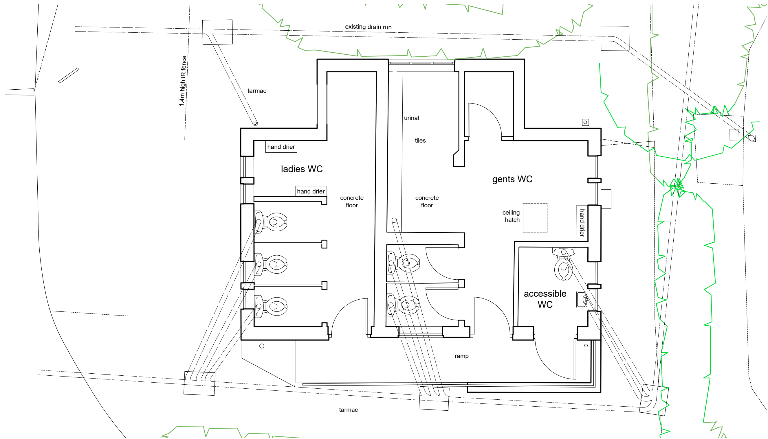
floor plan as existing 1:50
