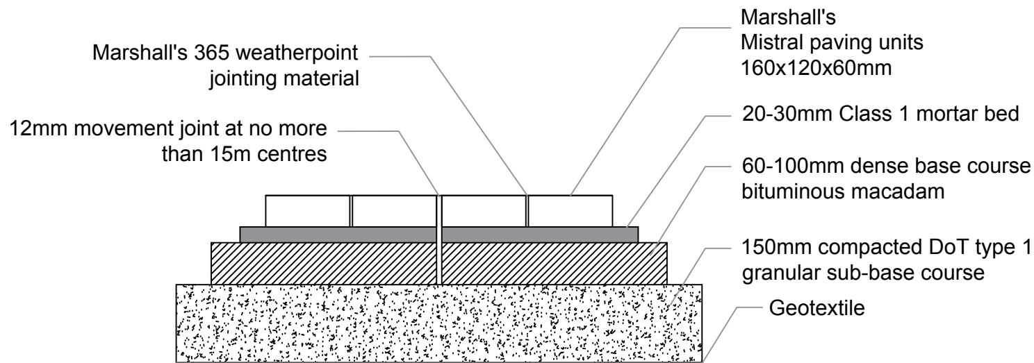
LOCK PAVING DETAIL
