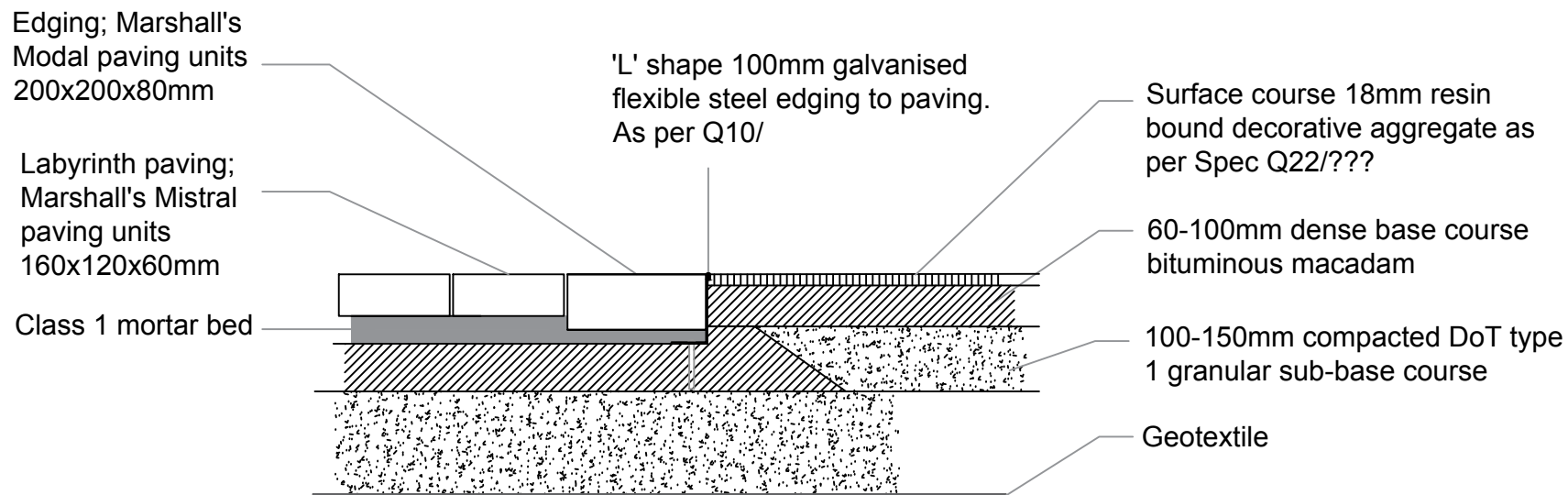
PAVING JUNCTION DETAIL
