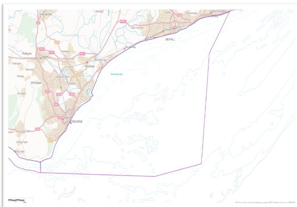
Figure 1: Lot 2 Acoustic Survey Area – Beachy Head East MCZ – Inshore East
