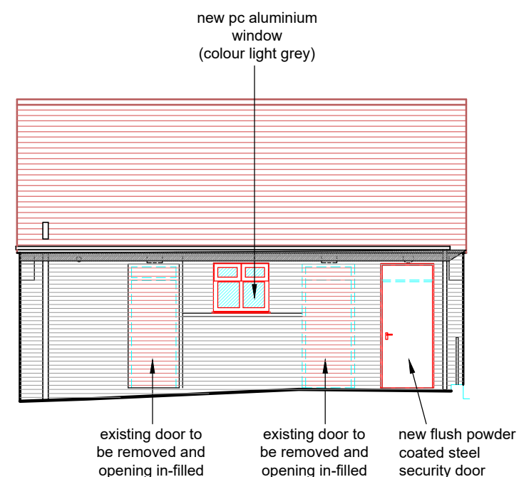
south facing elevation as proposed 1:100
