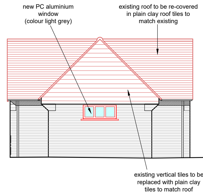
north facing elevation as proposed 1:100
