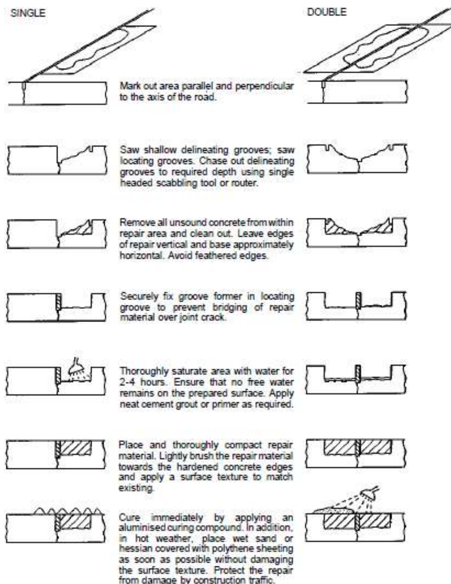
Figure 7/2-1 Procedure for thin bonded arris repairs to shallow spalling at joints (taken from Figure 8.2 of Concrete Pavement Maintenance Manual, 2001)
