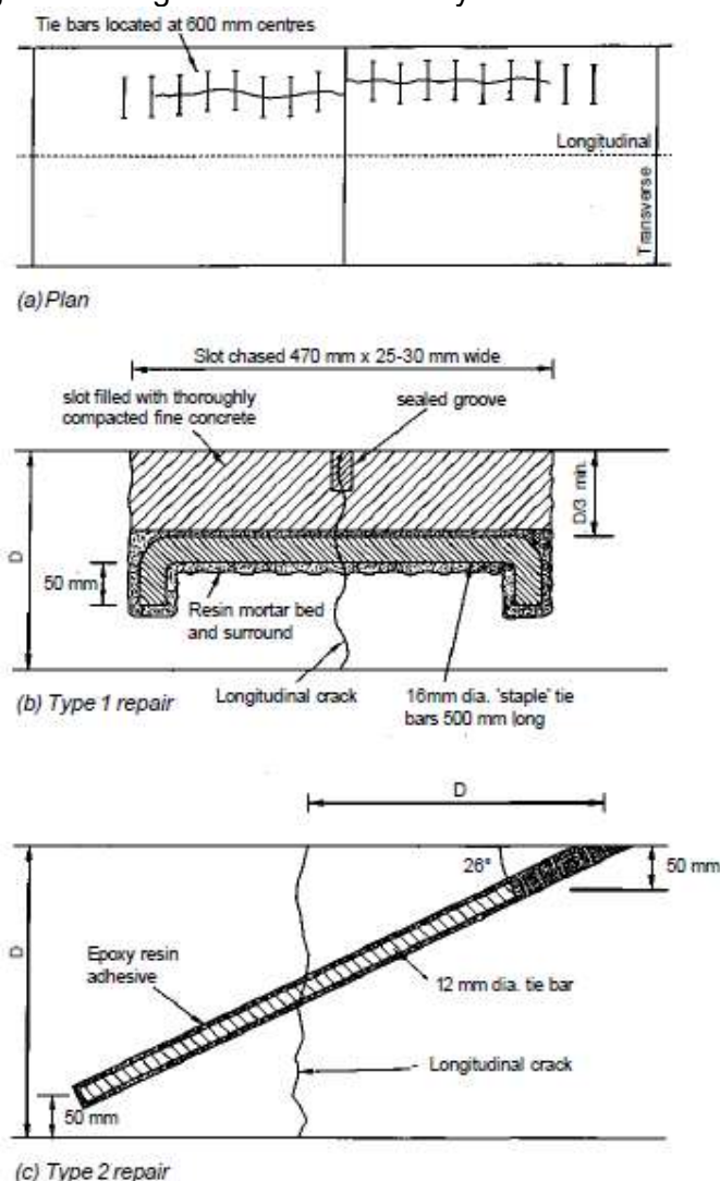
Figure 7/2-3 Stitched crack repairs (taken from Figure 8.4 of Concrete Pavement Maintenance Manual, 2001)
