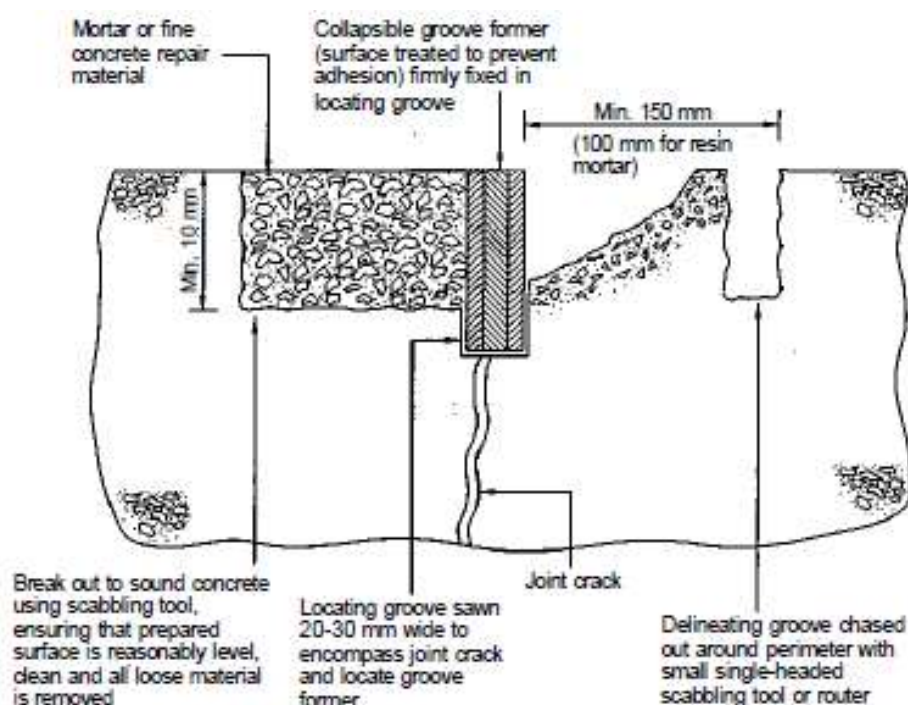
Figure 7/2-2 A thin bonded aris repair (taken from Figure 8.3 of Concrete Pavement Maintenance Manual, 2001)
