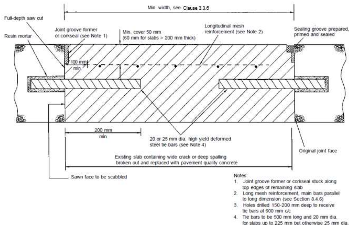
Figure 7/2-7 Transverse section through full-depth partial-width repair for JRC slabs (taken from Figure 8.8 of Concrete Pavement Maintenance Manual, 2001)
