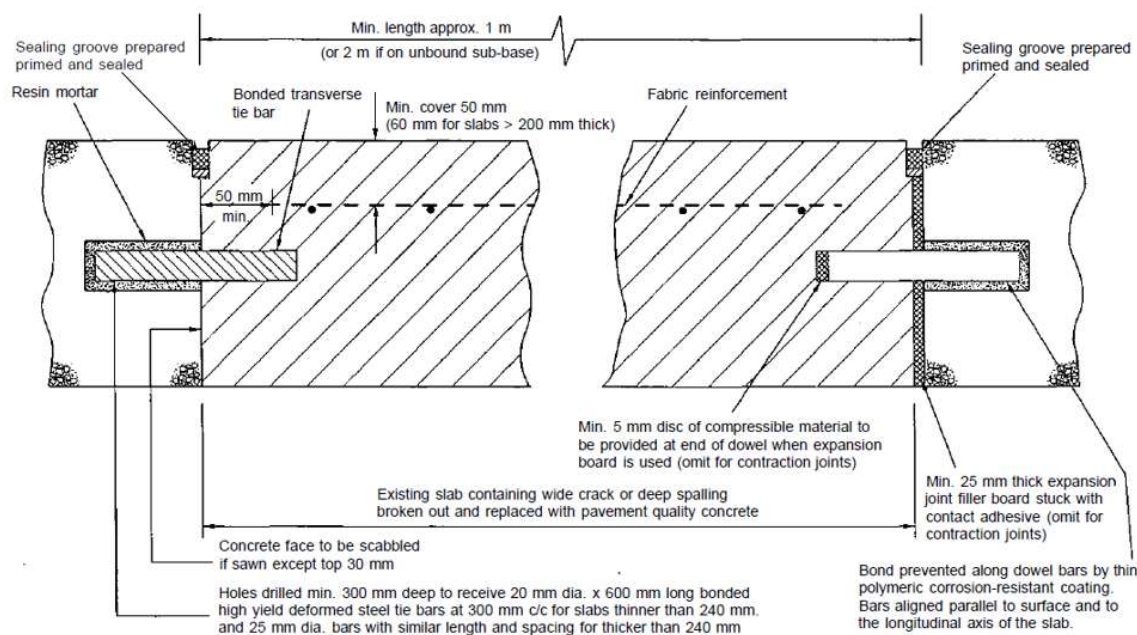
Figure 7/2-5 Longitudinal section through transverse full-depth repair adjacent to an existing transverse movement joint in URC pavement (taken from Figure 8.6 of Concrete Pavement Maintenance Manual, 2001)
