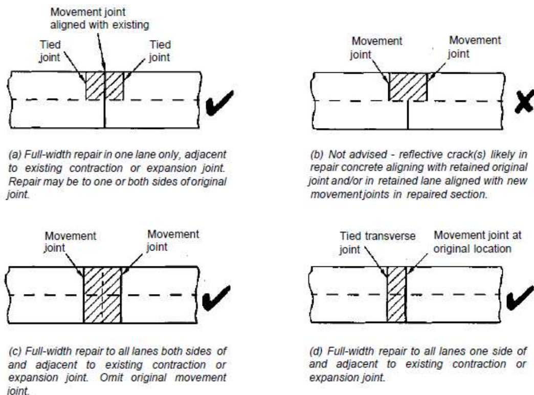
Figure 7/2-4 Full-depth repairs to jointed unreinforced concrete (URC) pavements (taken from Figure 8.5 of Concrete Pavement Maintenance Manual, 2001)
