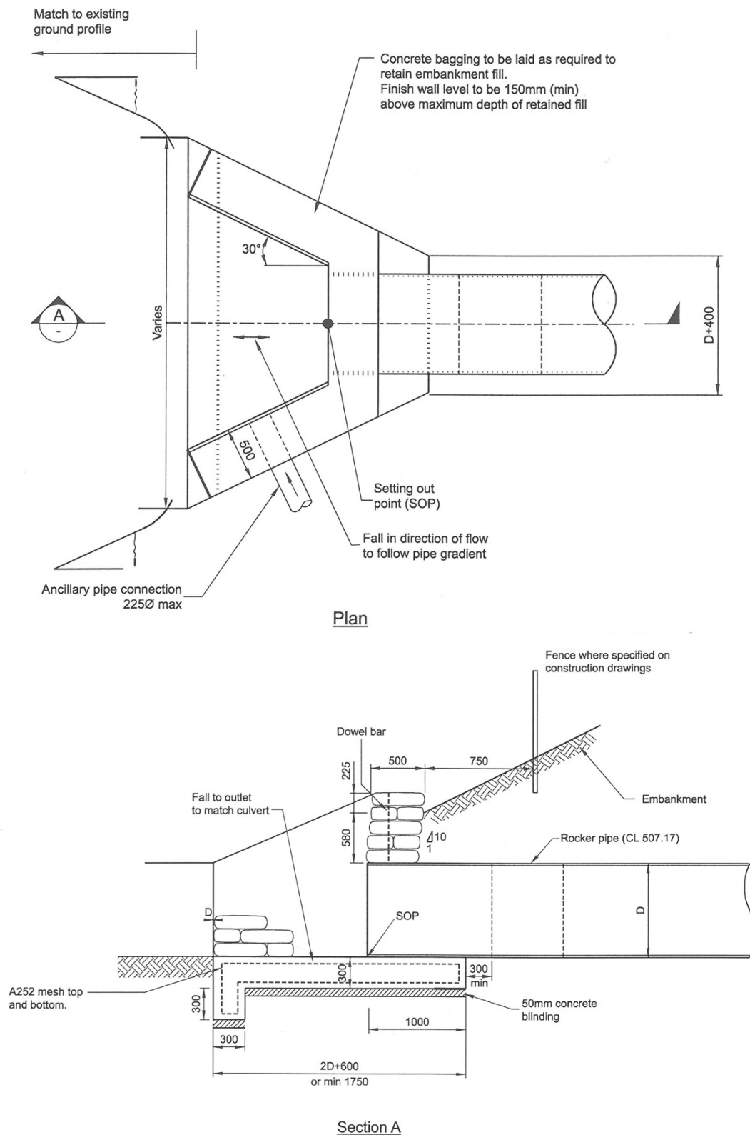
Figure 5-1 Headwall – Concrete Bagging
