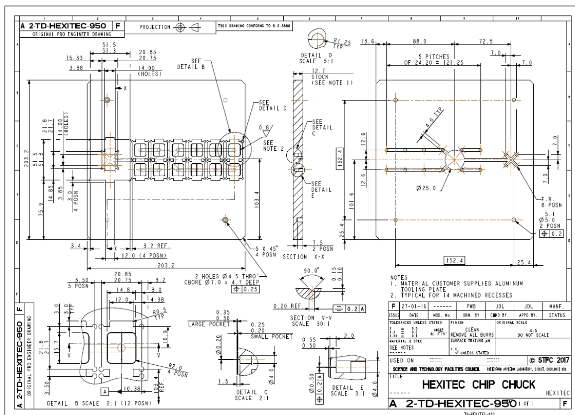
Figure 1: Engineering drawing for a typical heated work holder chuck.
